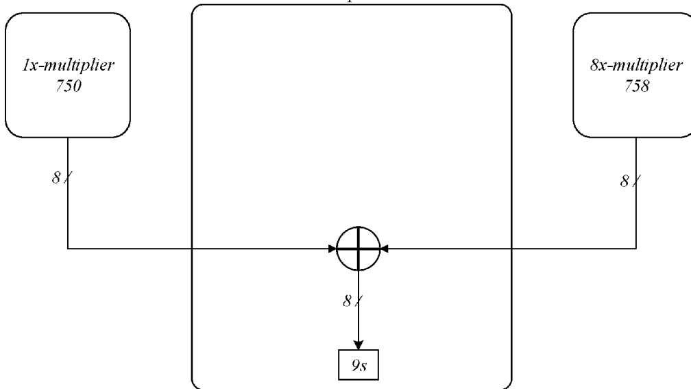
9x-multiplier 760
