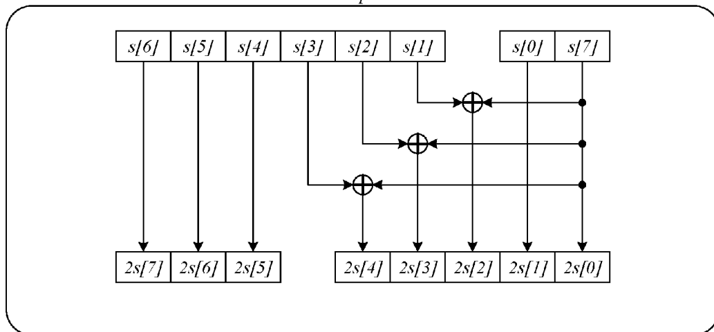
2x-multiplier 752
