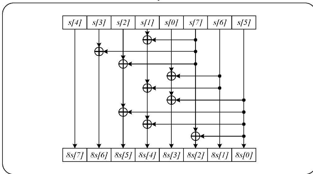
8x-multiplier 758
