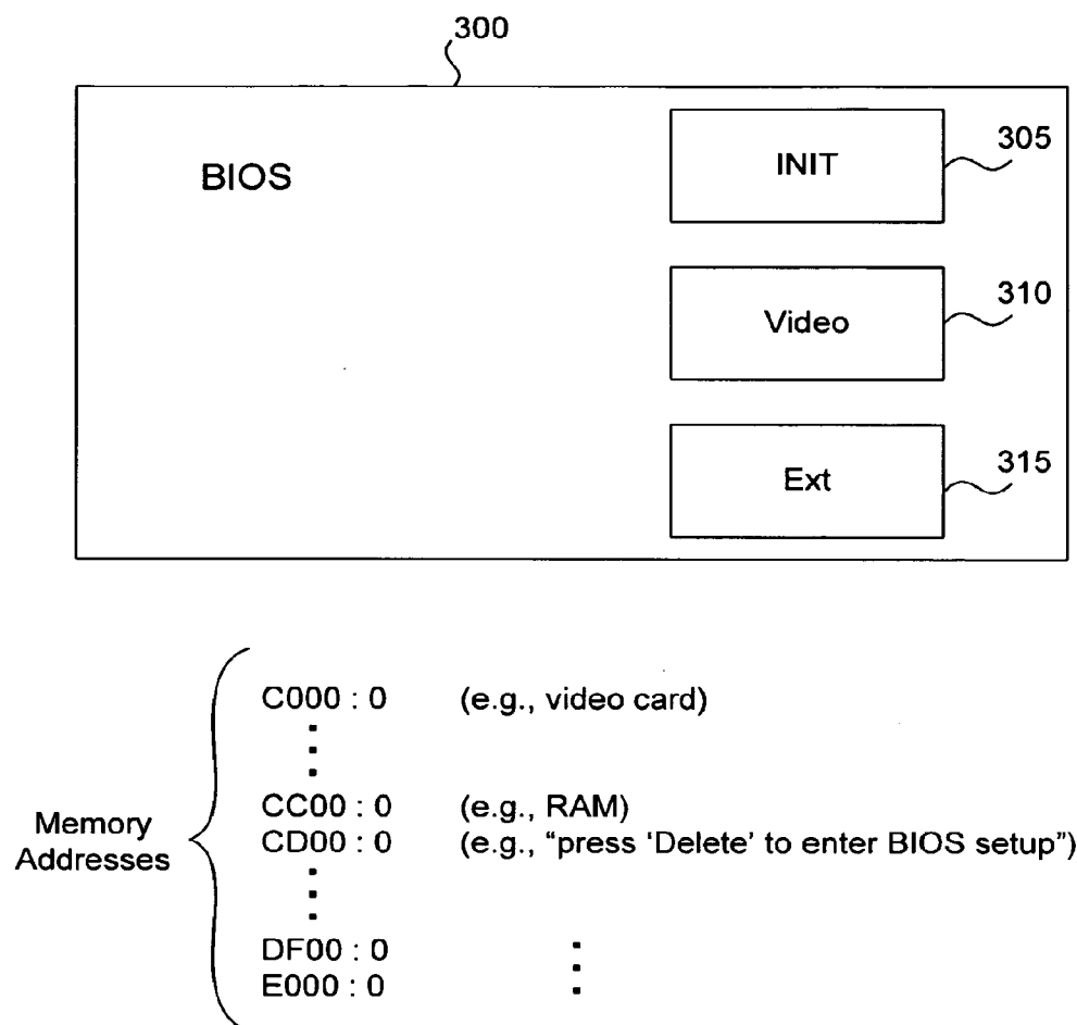
FIG. 3 (PRIOR ART)
