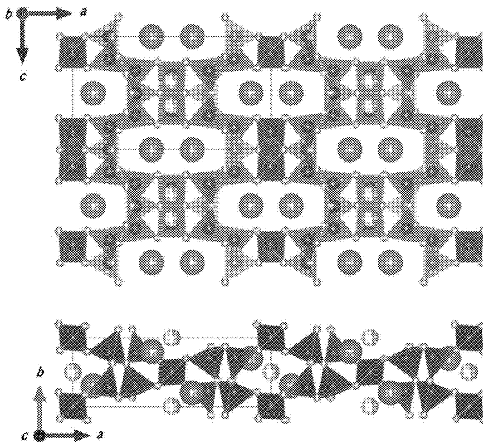
Crystal structure of \text{Li}_1\text{Ba}_2\text{Al}_1\text{Si}_7\text{N}_{12}
