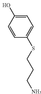
4-(3-Amino-propylsulfanyl)-phenol
