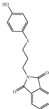
2-[3-(4-Hydroxy-phenylsulfanyl)-propyl]-isoindole-1,3-dione
