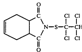
bis-N-[(1, 1, 2, 2-tetrachloroethyl)thio]-4-cyclohexene-1,2-dicarboximide
