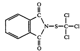
N-trichloromethylthio phthalimide
