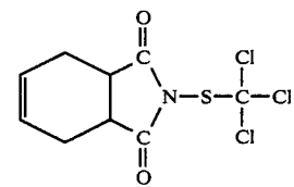
N-trichloromethylthio-4-cyclohexene-1,2-dicarboximide
