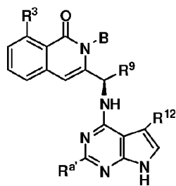
Formula XVI-A1
