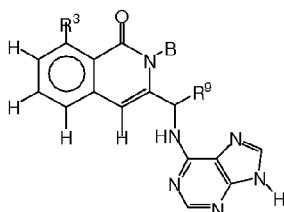
Formula V-A
