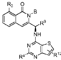
Formula XXI-A2
