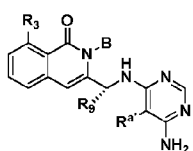
Formula XXII-A2
