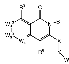
Formula XXIV-B
