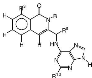
Formula VII-A
