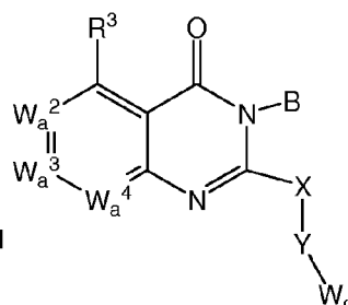
Formula XXIX
