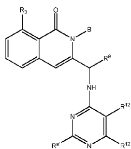
Formula XVII-A
