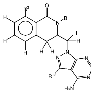
Formula XXVI-A
