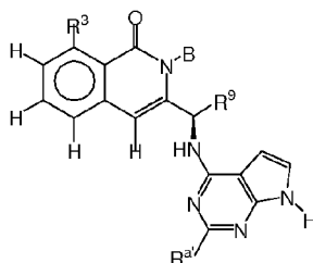
Formula XIII-A1
