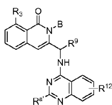
Formula XIX-A
