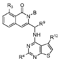
Formula XX-A
