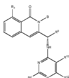
Formula XVII-A2
