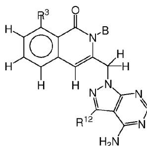
Formula IV-A
