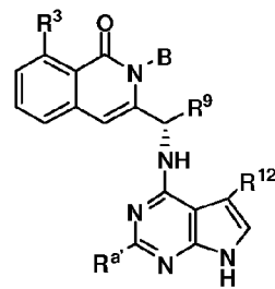
Formula XVI-A2
