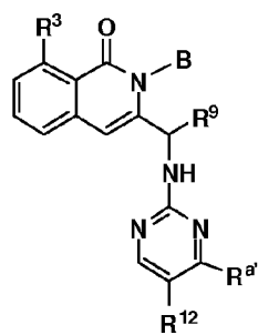
Formula XVIII-A
