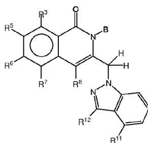
Formula XXVII-A
