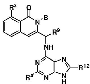
Formula XV-A
