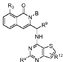
Formula XXI-A
