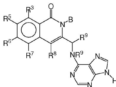
Formula XXVII-C
