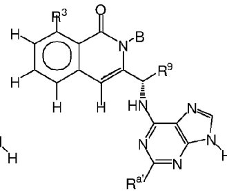
Formula VIII-A2
