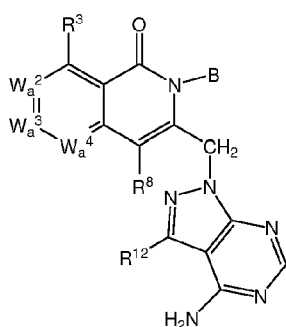
Formula XXIII-B
