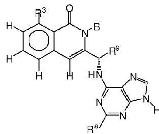
Formula X-A2
