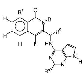
Formula XIII-A
