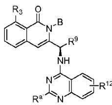
Formula XIX-A2
