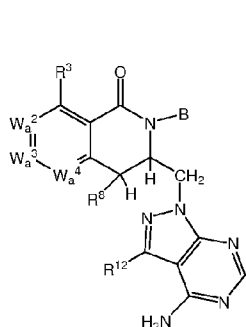
Formula XXIII-A
