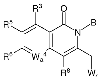
Formula XXVIII
