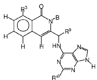
Formula X-A
