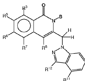
Formula IV
