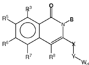
Formula XXVII
