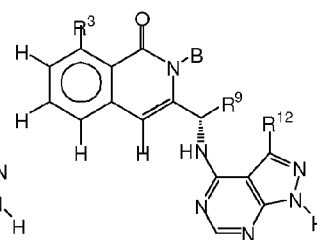
Formula XI-A2
