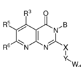
Formula XXIX-A
