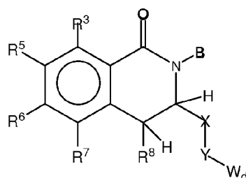
Formula XXVI
