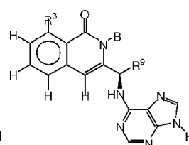
Formula V-A1
