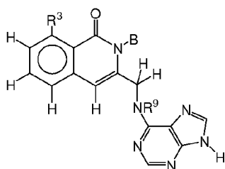
Formula V-B
