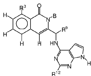
Formula XII-A
