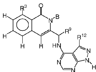
Formula IX-A
