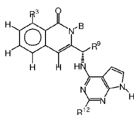
Formula XII-A1
