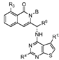
Formula XX-A3
