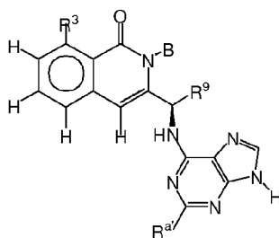
Formula X-A1
