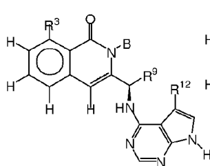
Formula IX-A1
