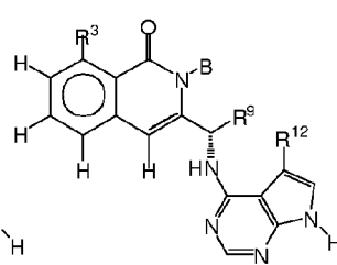
Formula IX-A2
