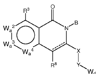
Formula XXV
