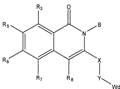
Formula (Ib),
