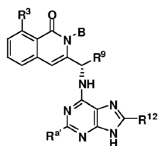
Formula XV-A2
