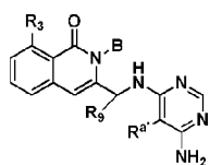
Formula XXII-A
