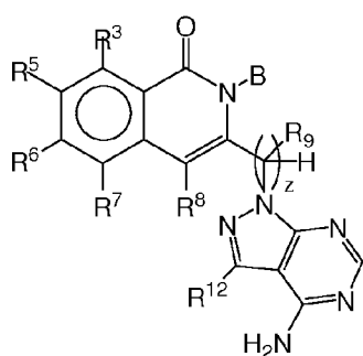
Formula XXVII-B
