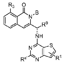
Formula XXI-A3
