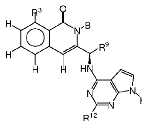
Formula XII-A2
