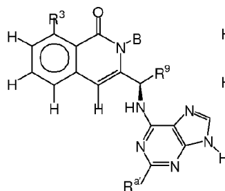
Formula VIII-A1
