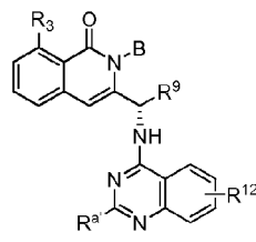
Formula XIX-A3
