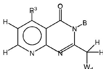
Formula XXIX-A1
