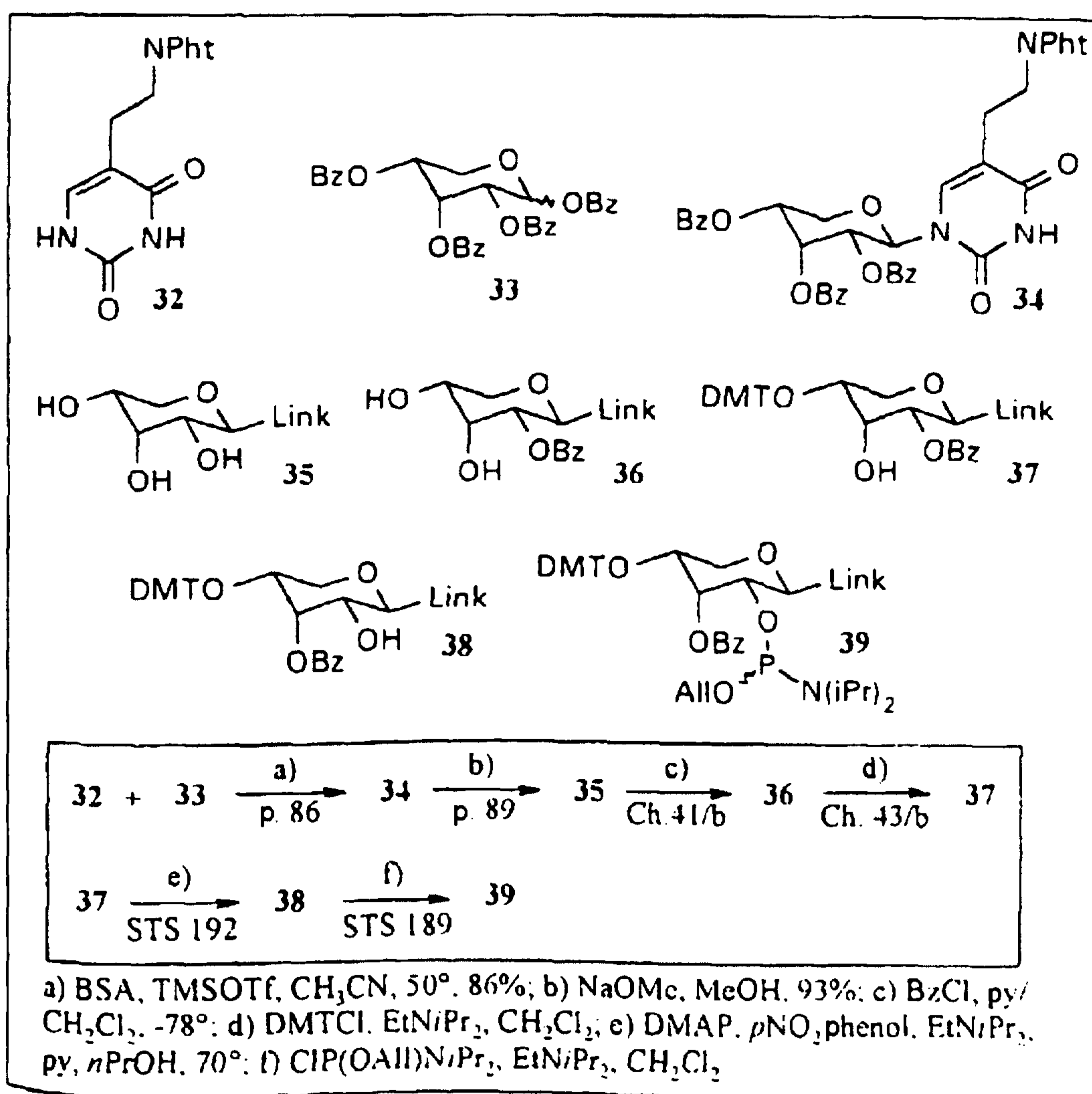
Scheme 6: Synthesis of the linker phosphoramidite 39 .
