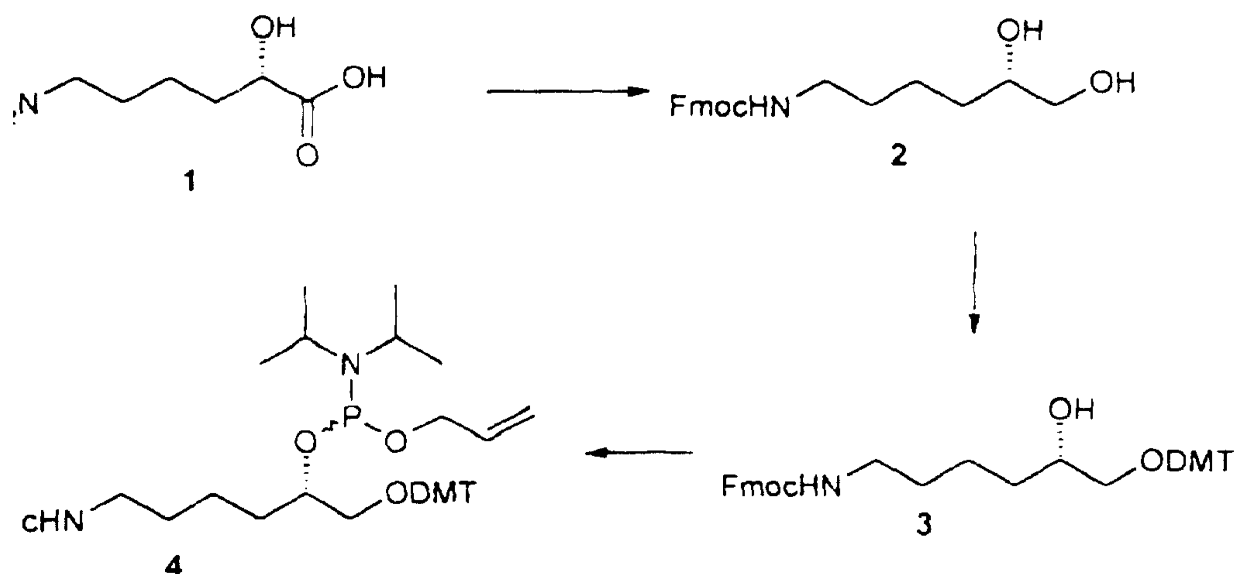
Scheme 7: Synthesis of the lysine linker
