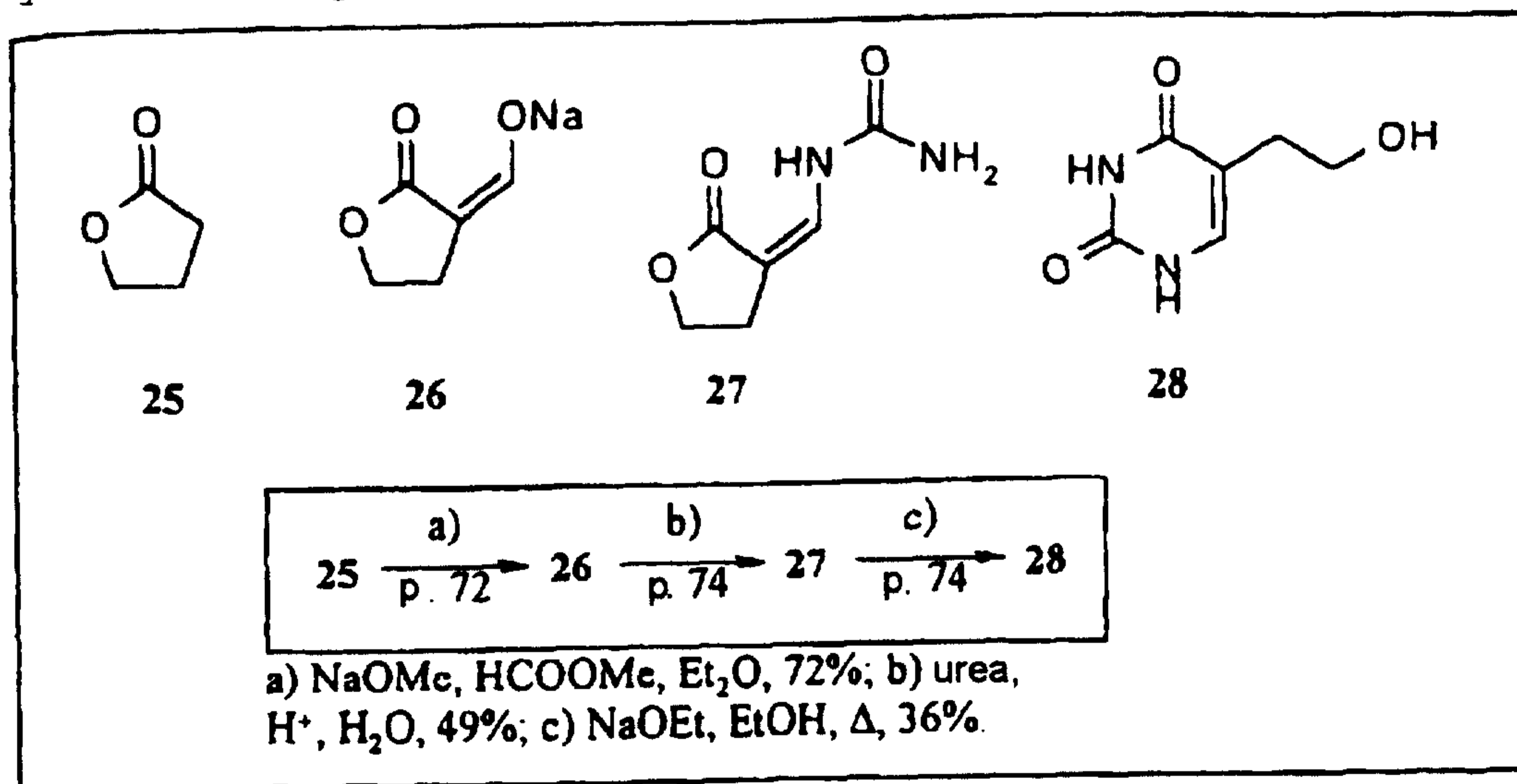
Scheme 4: Synthesis of hydroxyethyluracil 28 .
