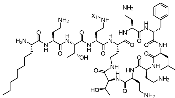
Nonanamide-Dab-Thr-Dab(NH 2 )-Dab*-Dab-[D-Phe]-Leu-Dab-Dab-Thr*
