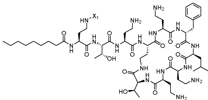
H 2 N-Dab-Thr-Dab-Dab*-Dab-[D-Phe]-Leu-Dab-Dab-Thr*
