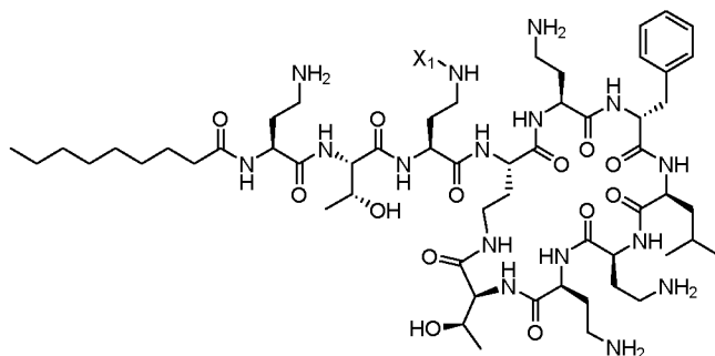
Nonanamide-Dab-Thr-Dab(NH 2 )-Dab*-Dab-[D-Phe]-Leu-Dab-Dab-Thr*
