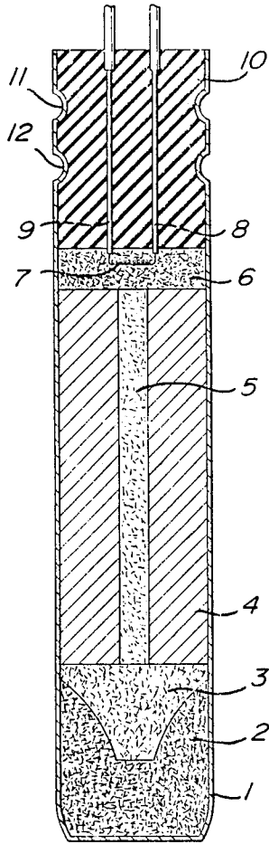
FIG. 1 PRIOR ART
