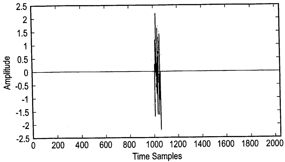
Fig. 3a: Burst Duration of 5 \mu sec; x(t)
