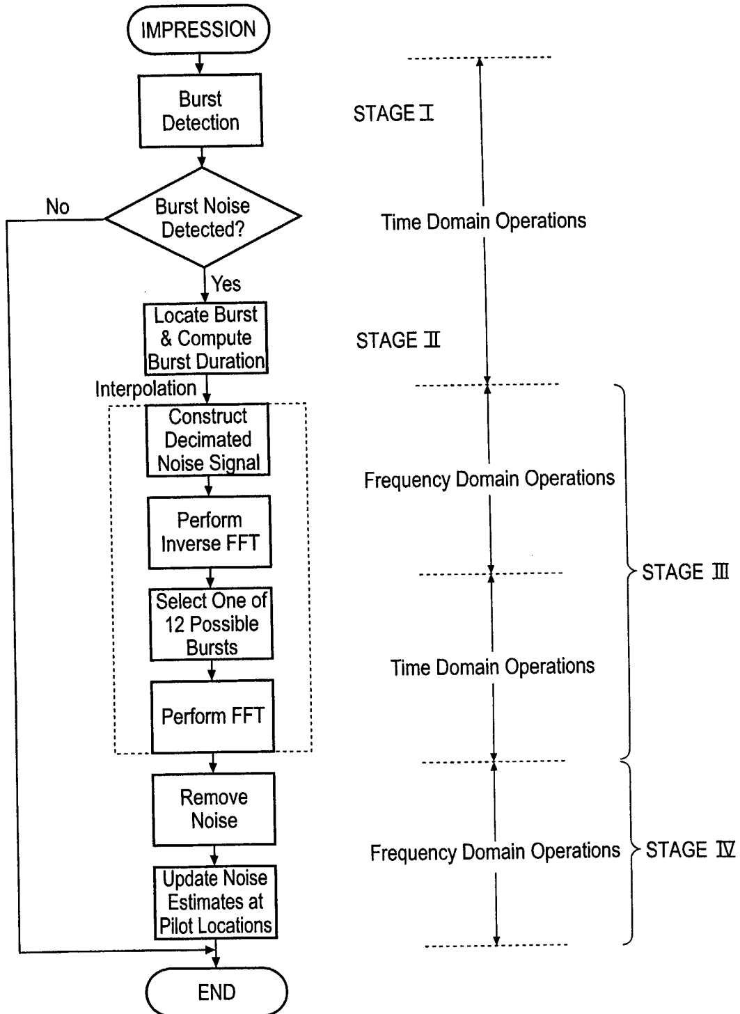
Fig. 5: Flow Chart of IMPRESSION
