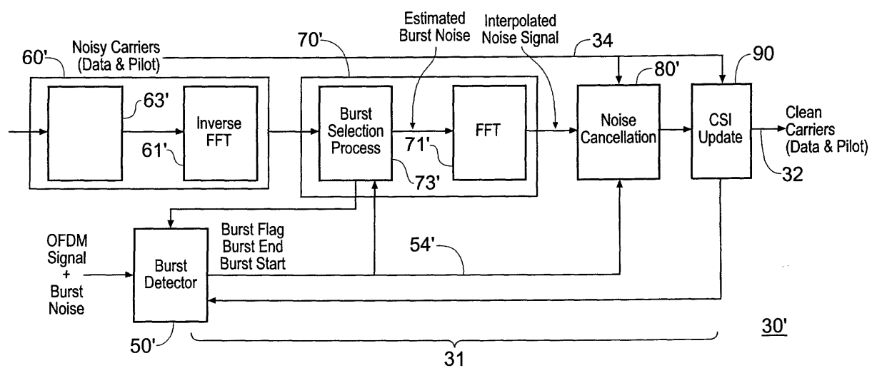
Fig. 4b: Frequency Domain Burst Noise Suppression Processor
