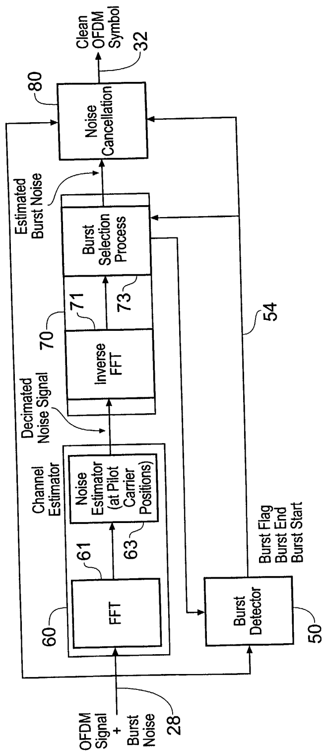
Fig. 4a: Time Domain Burst Noise Suppression Processor
