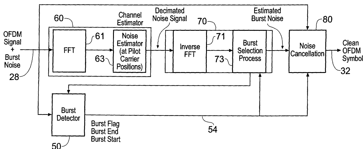
Fig. 4a: Time Domain Burst Noise Suppression Processor
