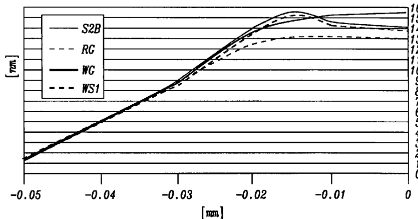
X-track Actuation Profile (2heater source = 30µm distance)
