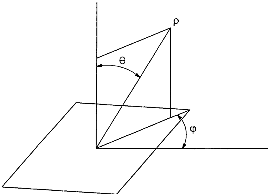
SPHERICAL SYSTEM OF COORDINATES
