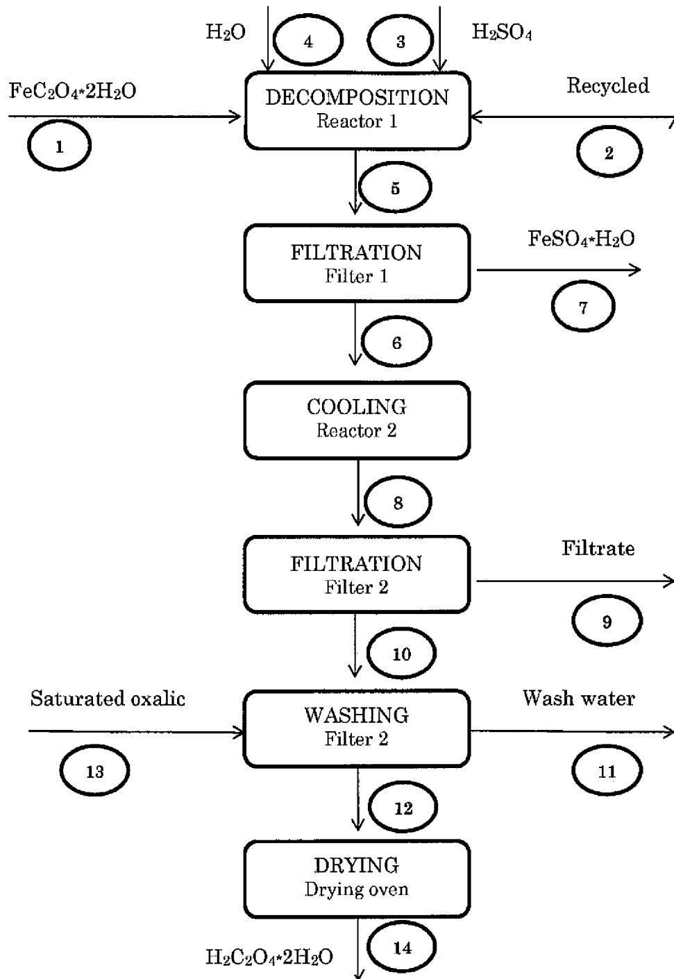
FLOW DIAGRAM OF OXALIC ACID RECOVERY FROM FERROUS OXALATE DIHYDRATE
