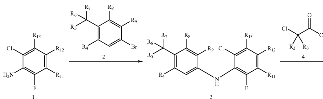
Scheme I
