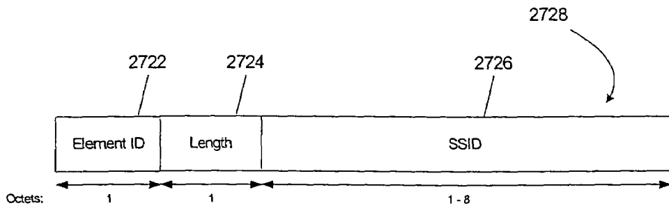
Figure 27B (SSID Information Element Format)
