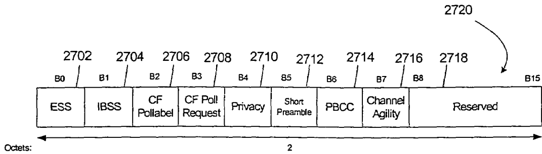
Figure 27A (Capability Information Fixed Field)
