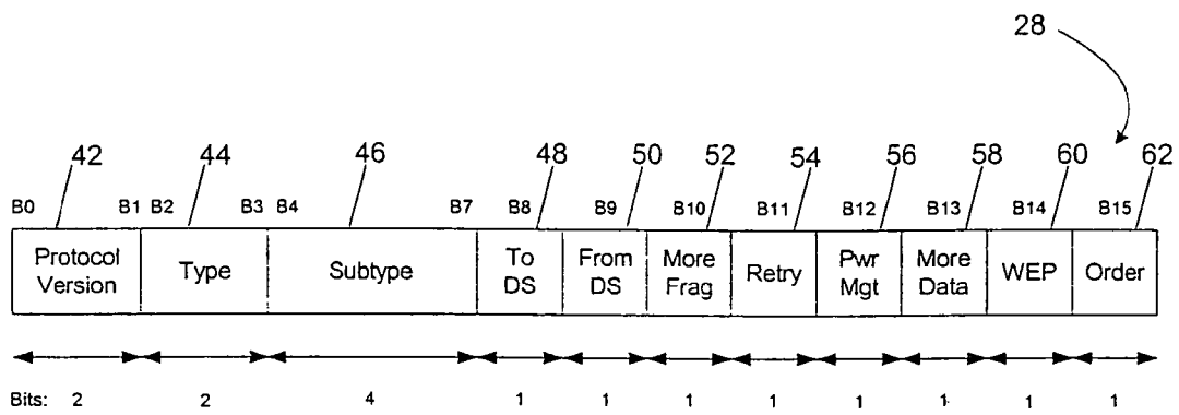
Figure 2B (Frame Control Field)
