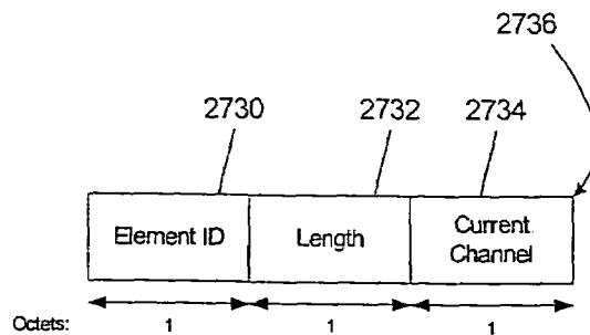
Figure 27C (DS Parameter Set Information Element Format)
