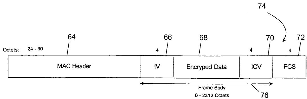
Figure 2C (WEP Encrypted Frame Format)
