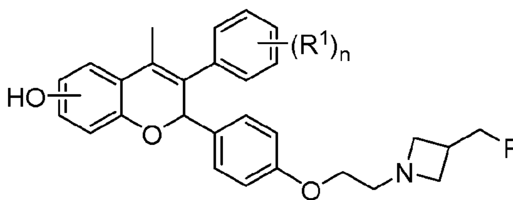
Formula (I)
