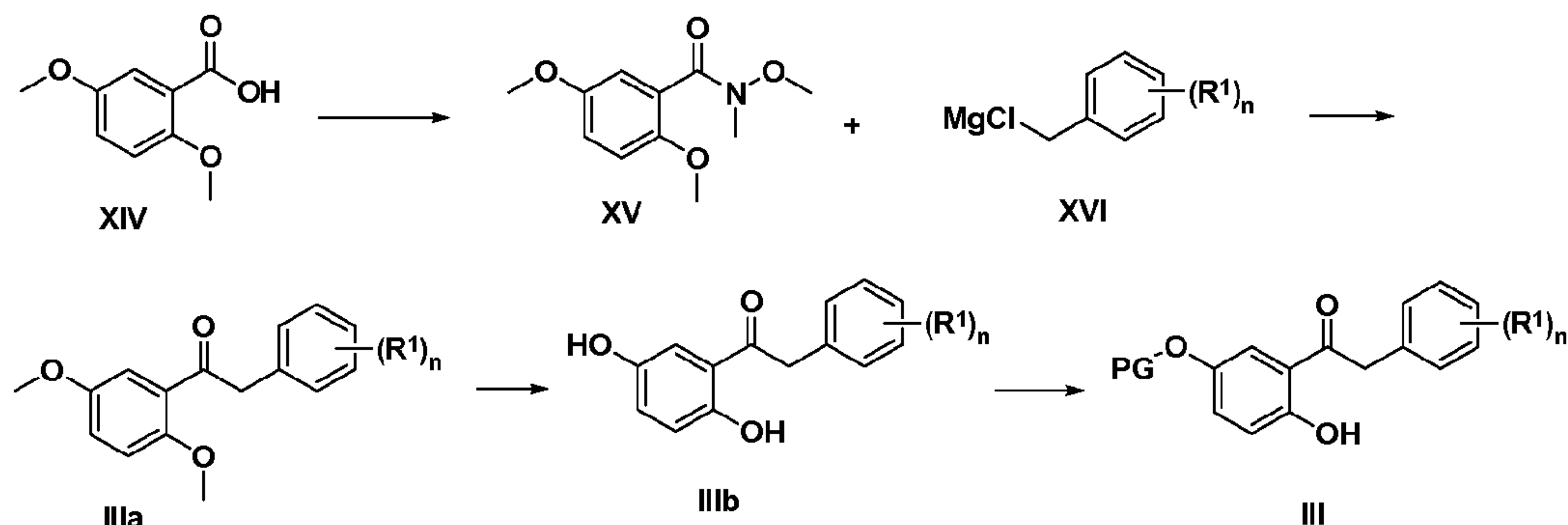
Scheme 4:
