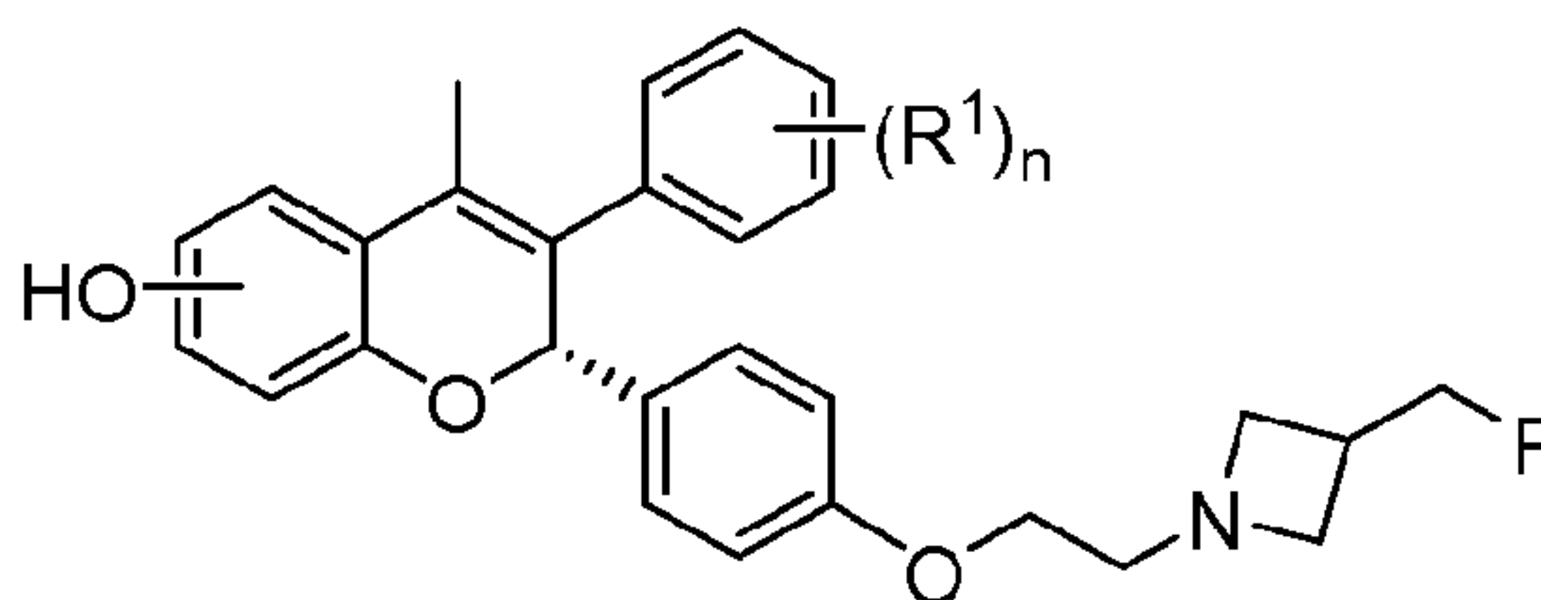
Formula (III)
