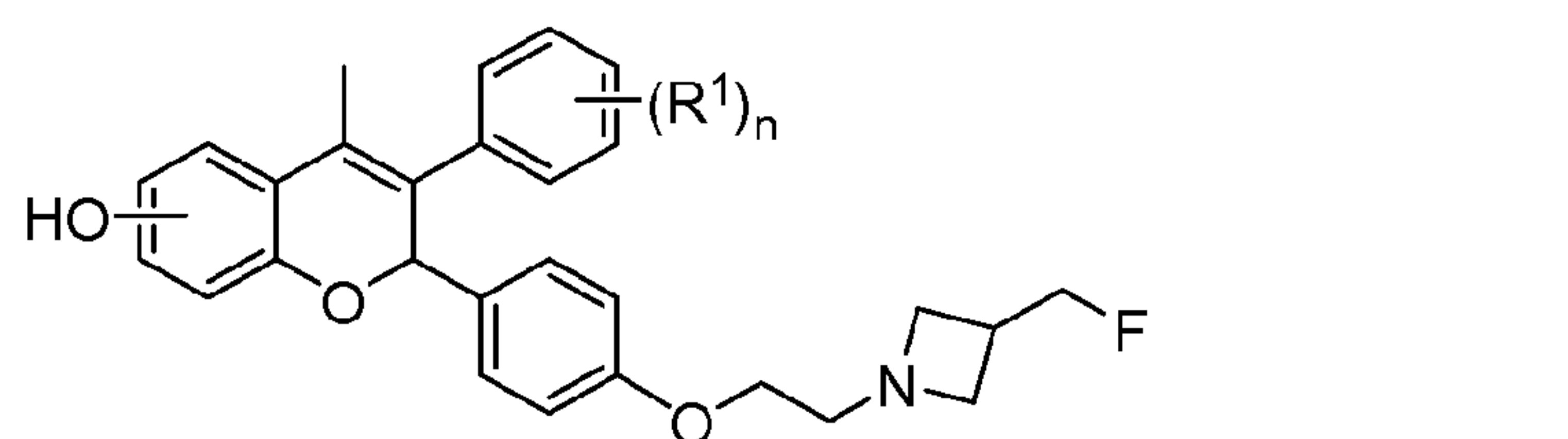
Formula (I)
