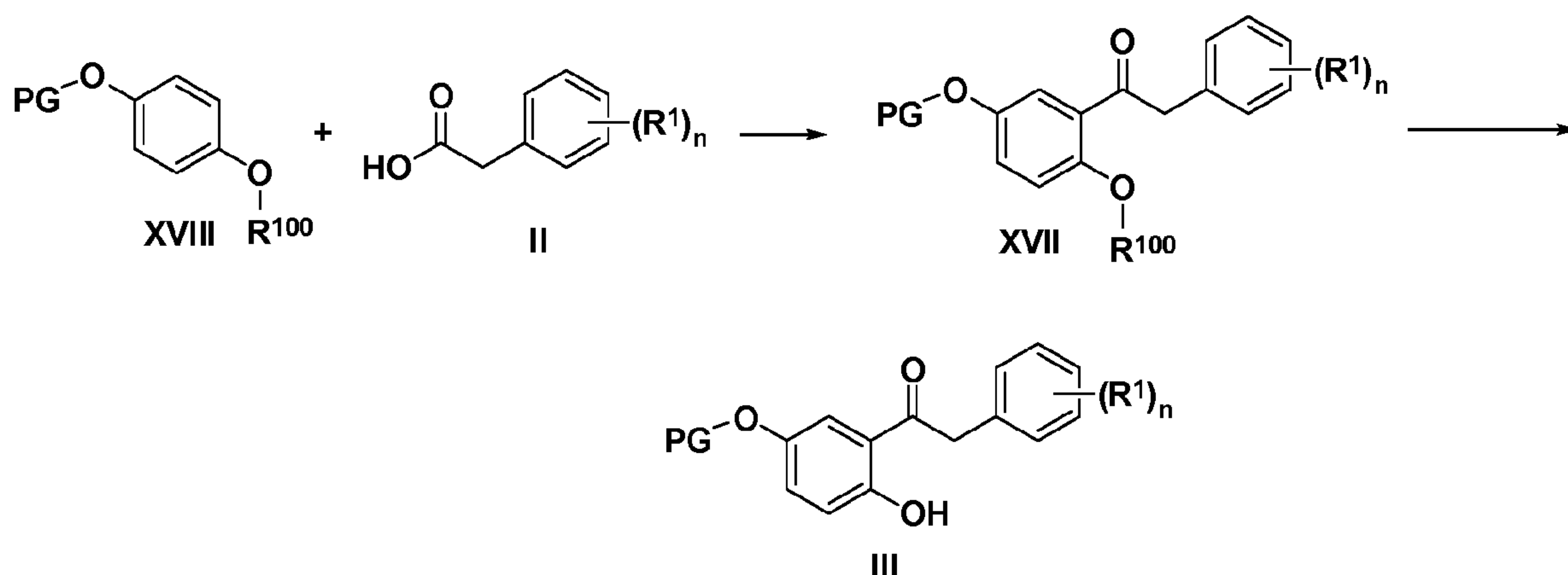
Scheme 5:
