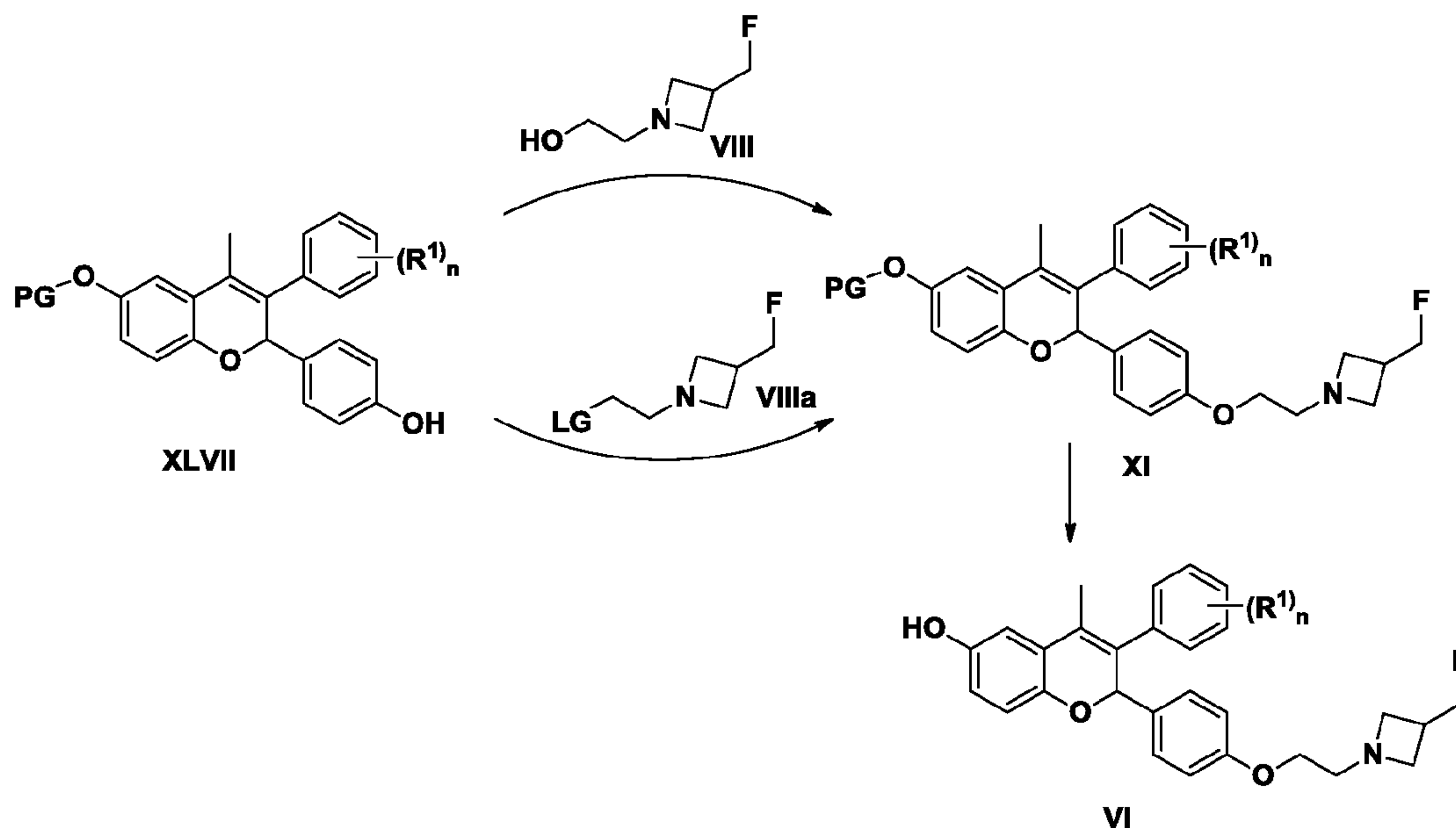
Scheme 13.
