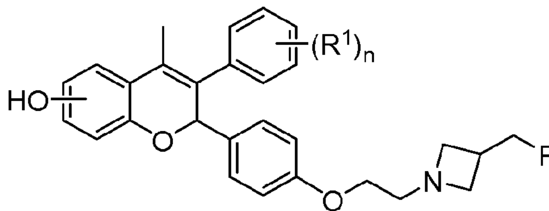
Formula (I)
