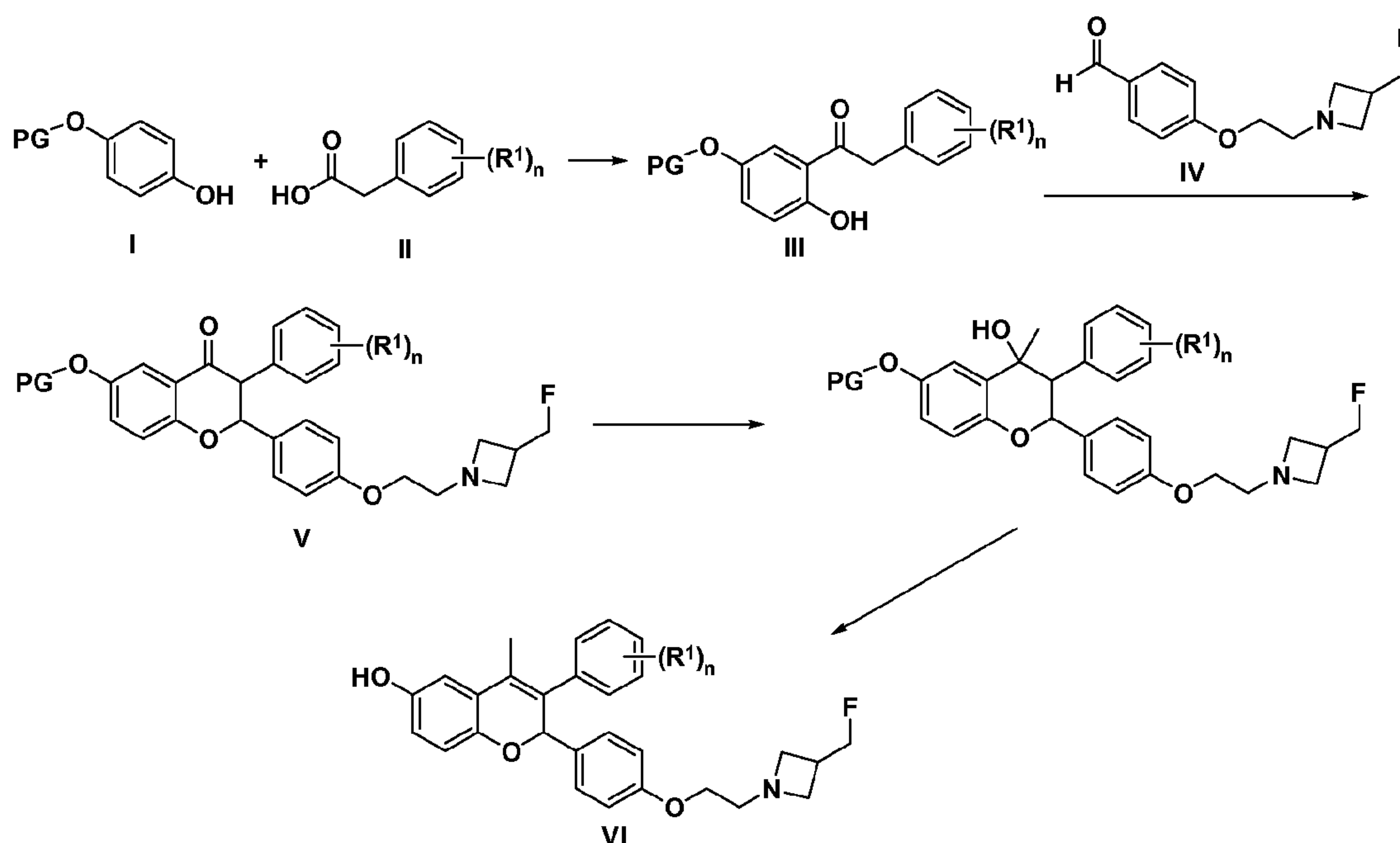
Scheme 1:
