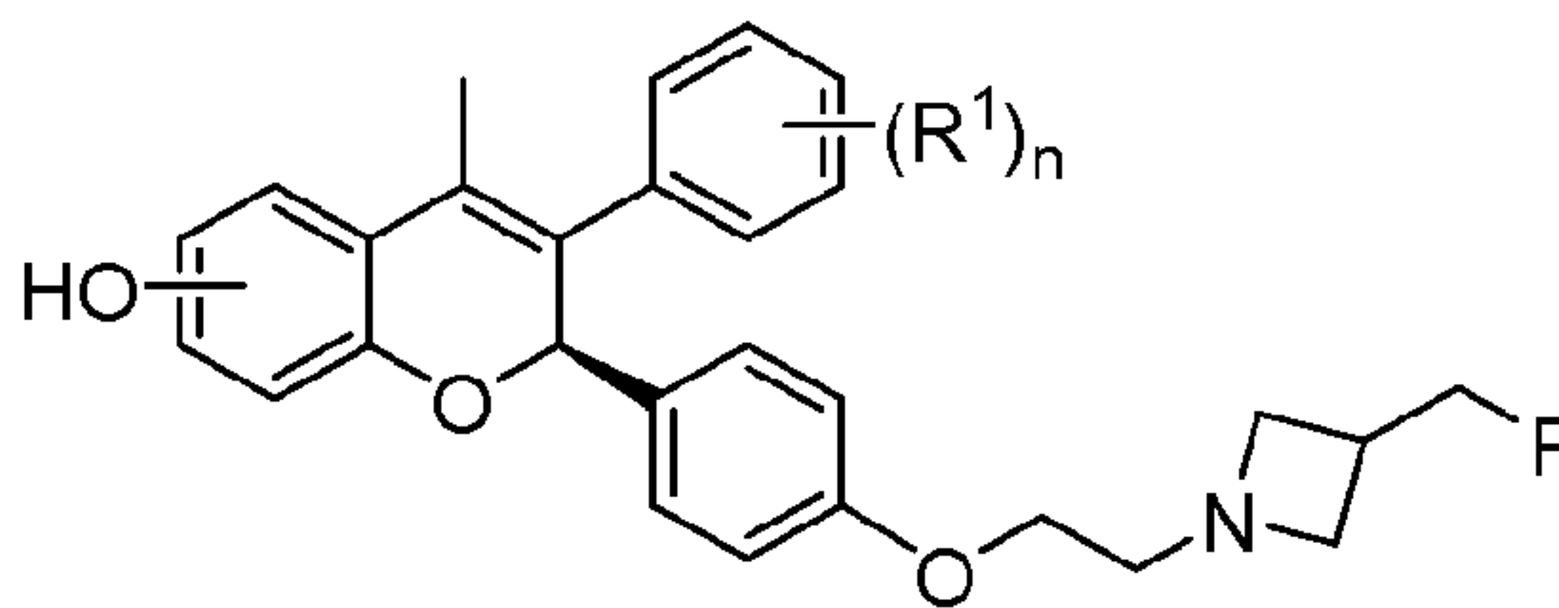
Formula (II)
