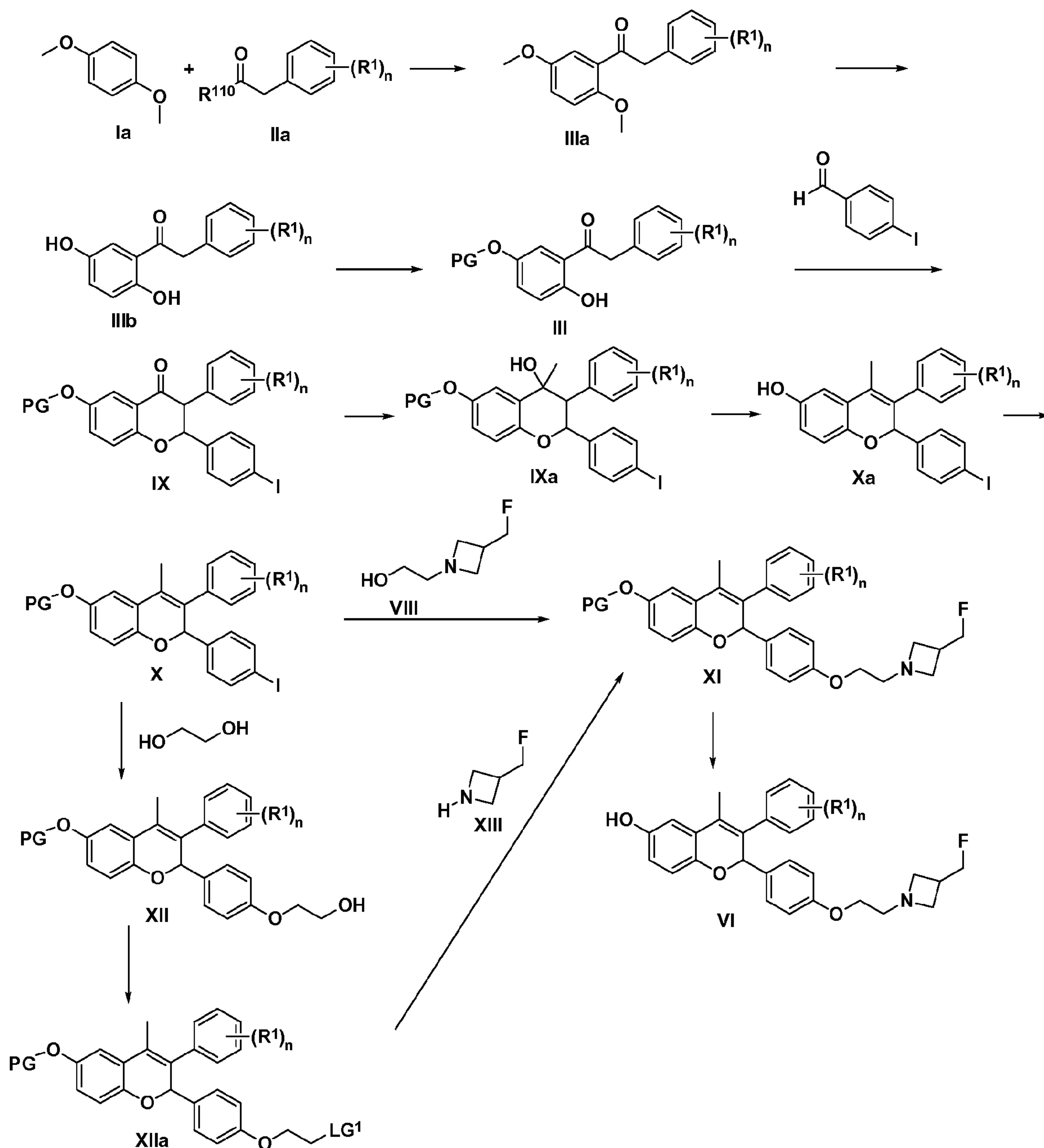
Scheme 3:
