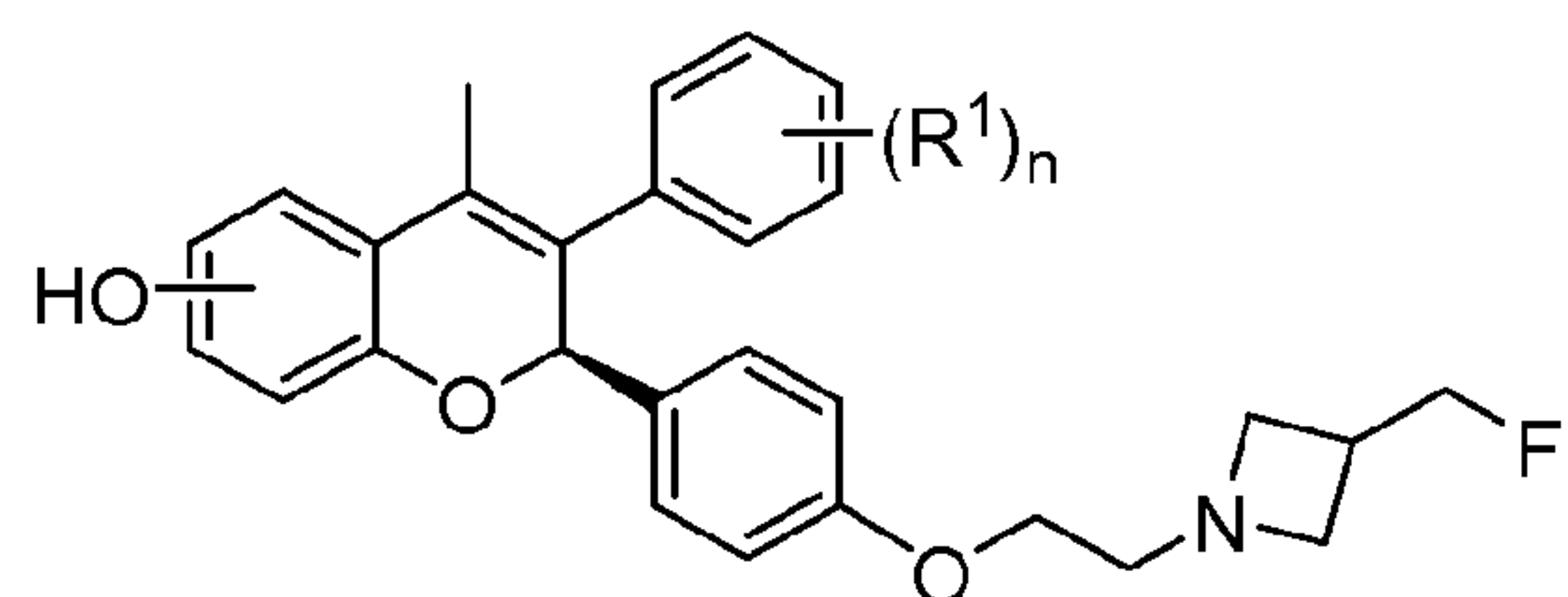
Formula (II)
