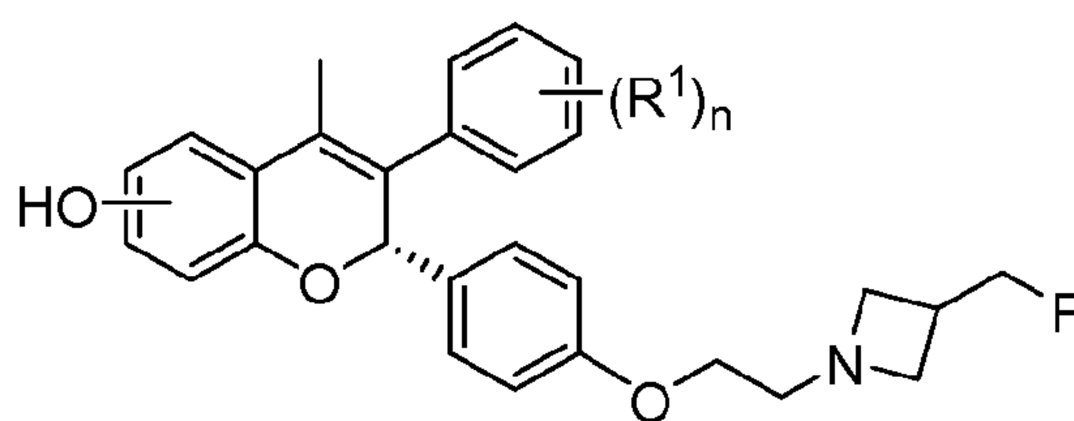
Formula (III)
