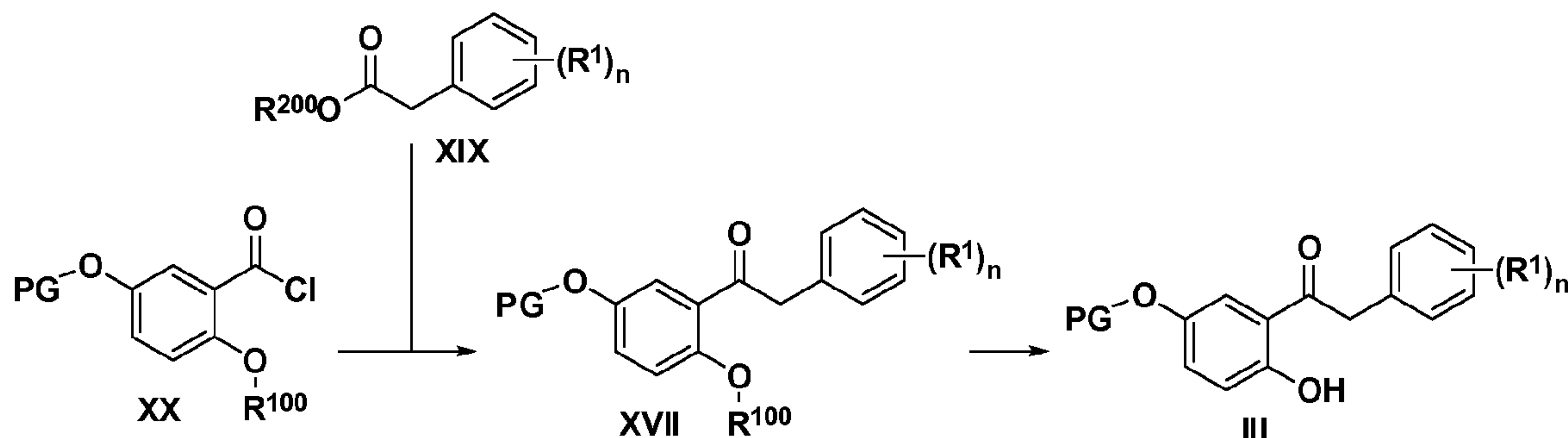
Scheme 6:
