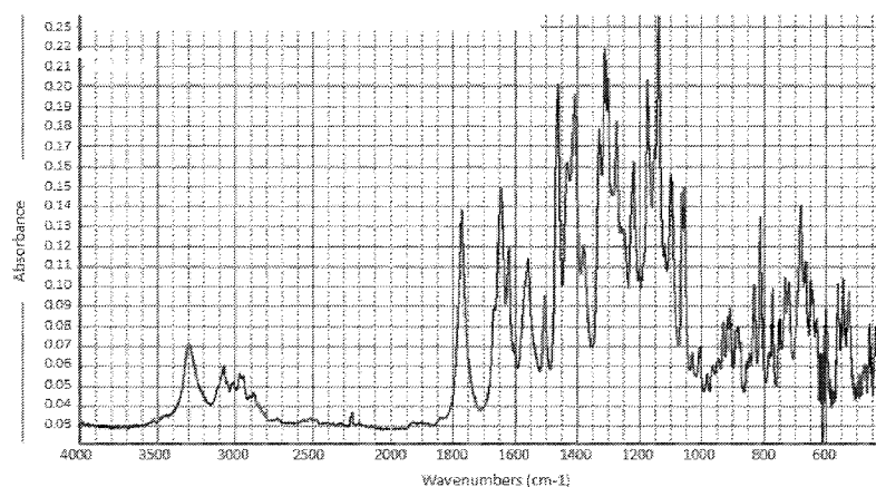
Infrared spectrometry (microATR) of ARN-509 Form B.
