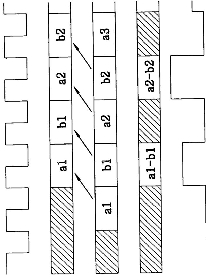
FIG. 6A SIGNAL READING TIMING FOR CCD 233
