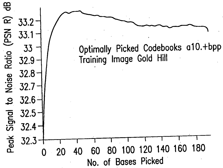
PSNR as successive bases are selected in a 14x14 separable codebook at a fixed rate of 0.4 bpp
