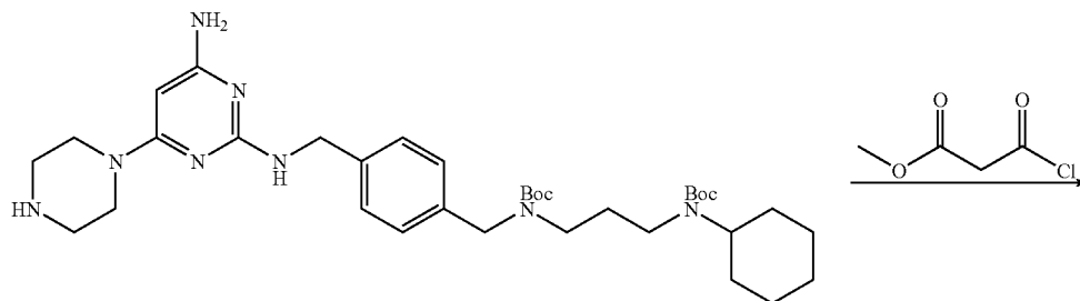
21-II
