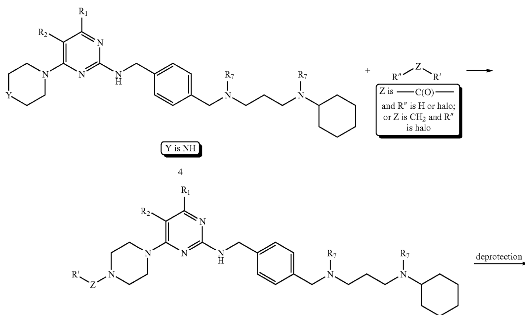
Scheme IV
