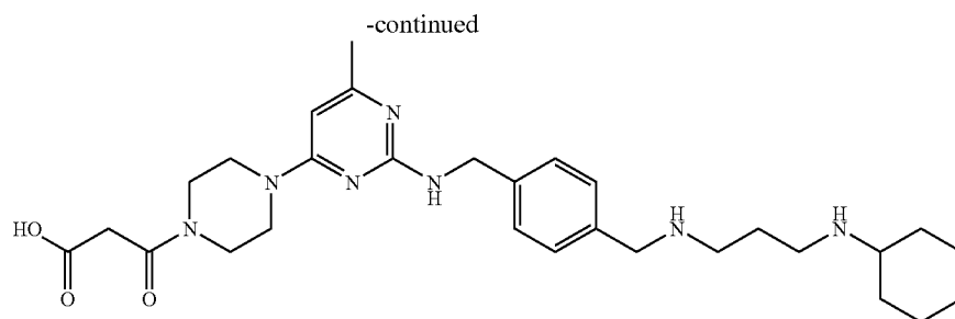
Compound 154
