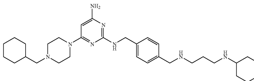
Compound 35
