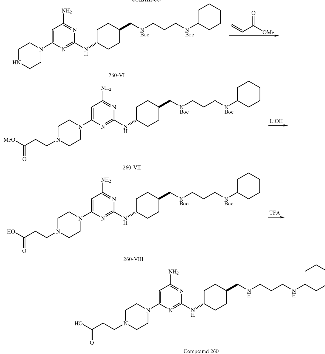
Compound 260
