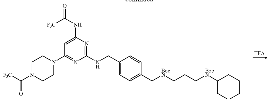
95-II
