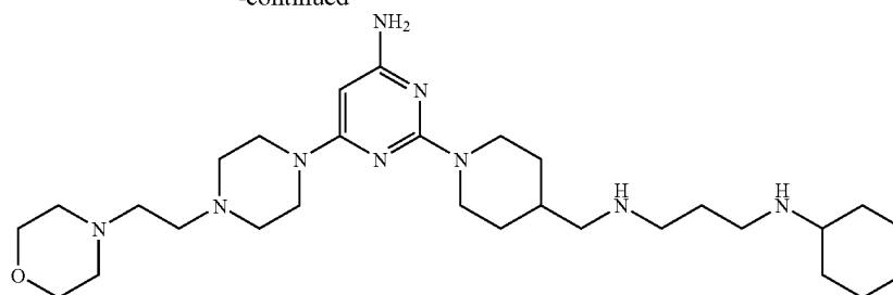
Compound 227
