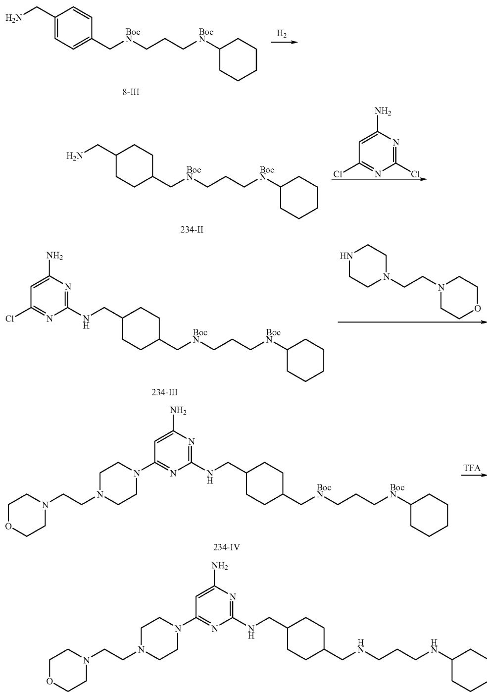
Compound 234
