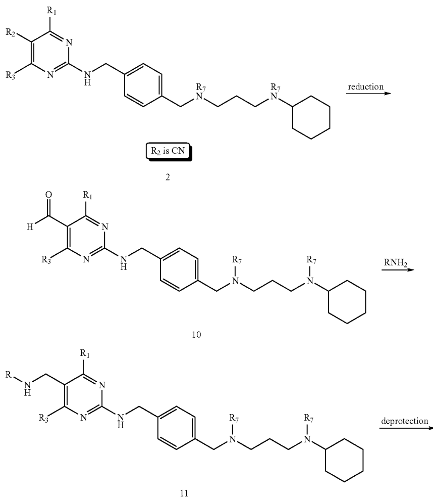
Scheme III
