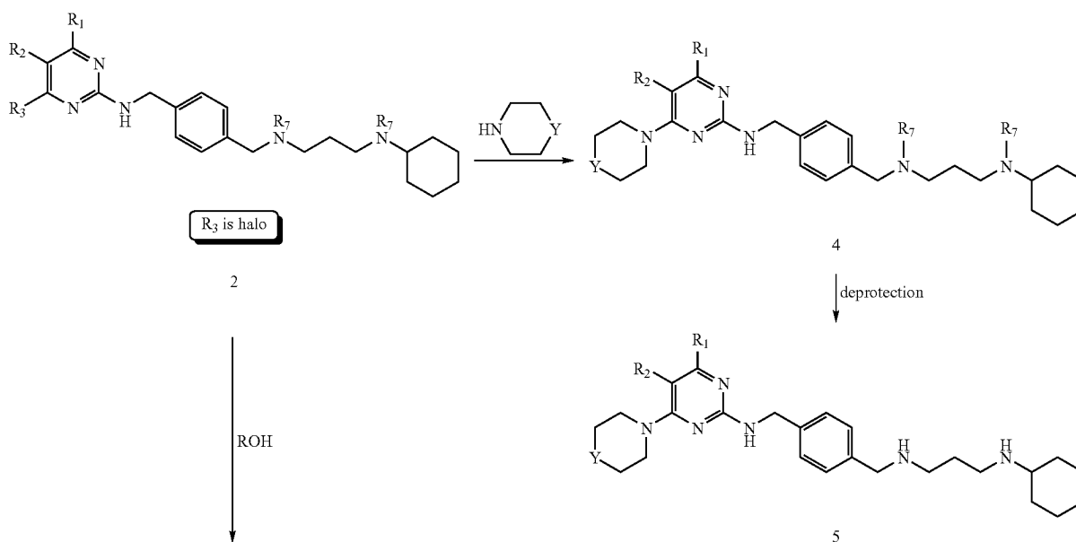
Scheme II
