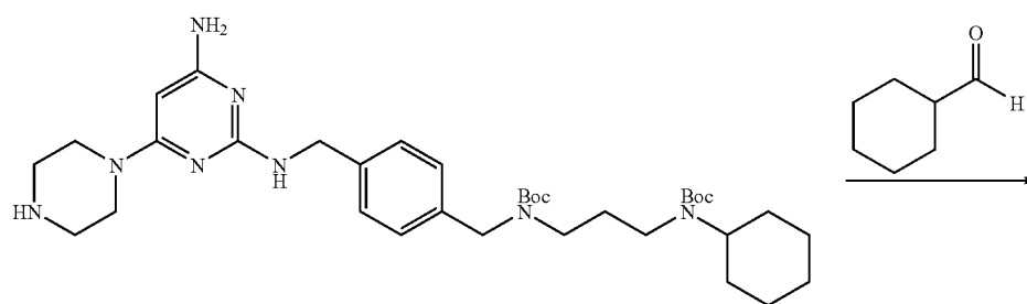
35-I
