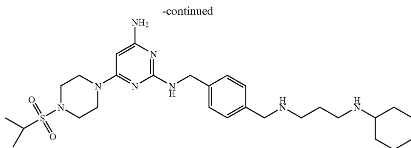
Compound 109
