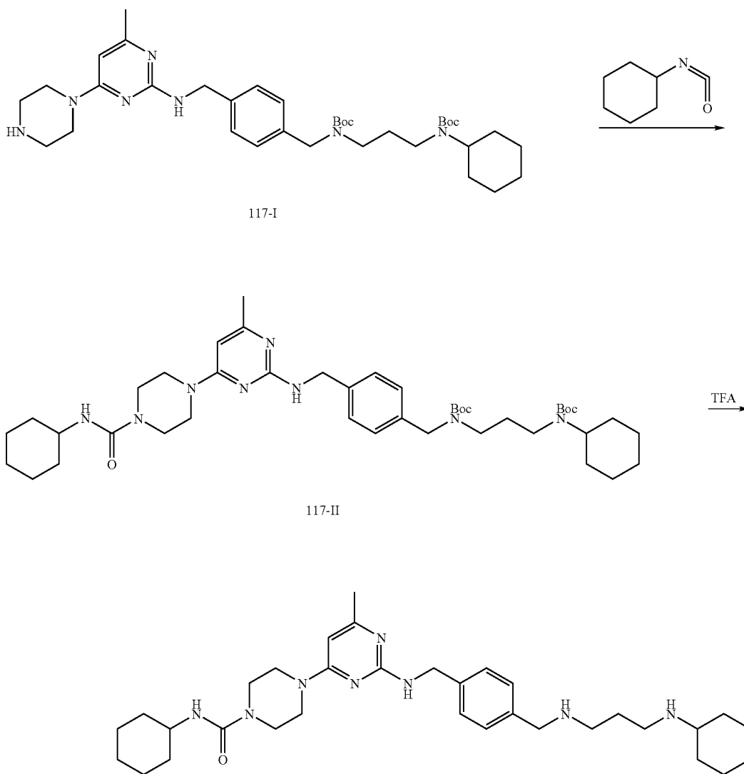
Compound 117
