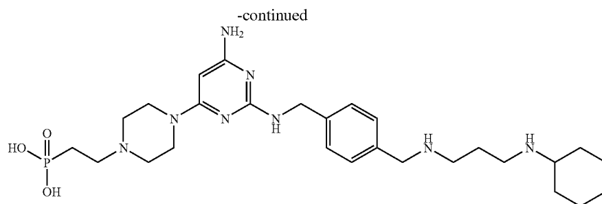
Compound 230
