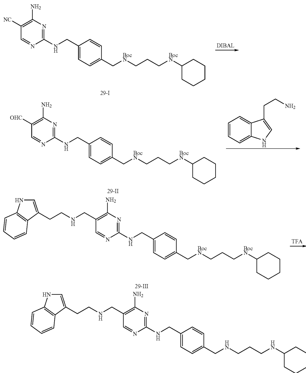
Compound 29
