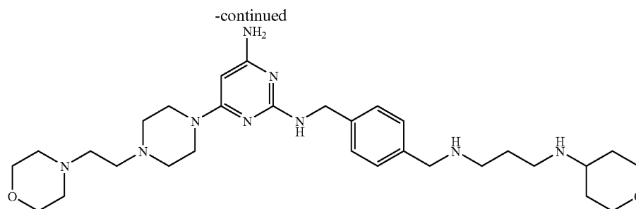
Compound 204
