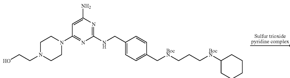
22-II
