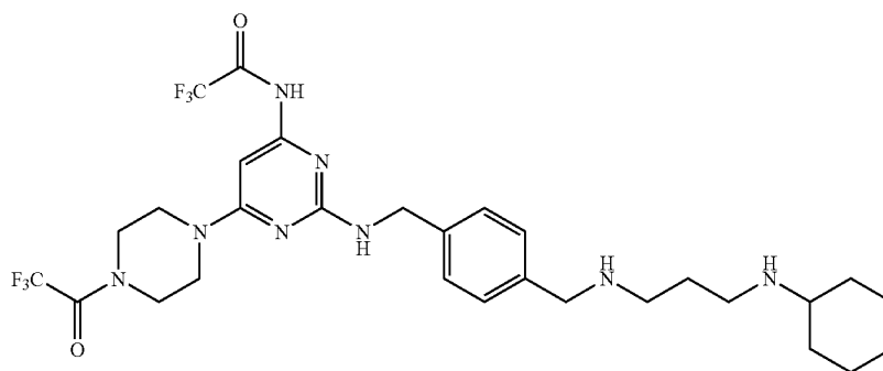
Compound 95
