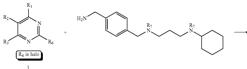
Scheme I
