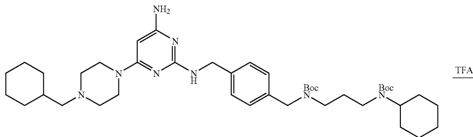
35-II
