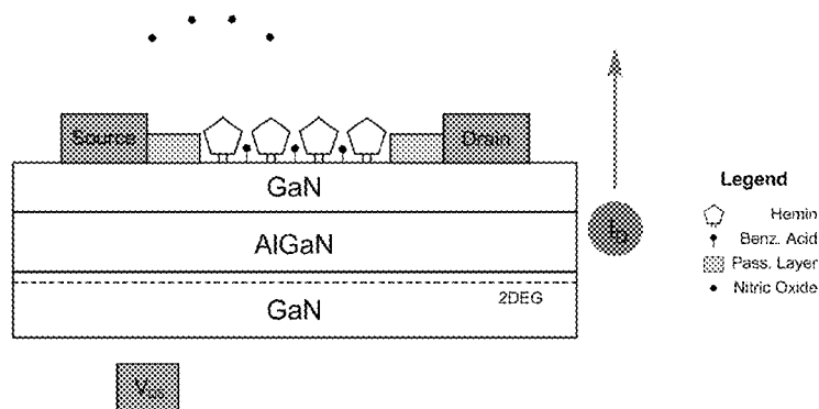
Schematic of Functionalized GaN-AlGaIn HFET
