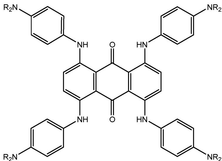
Anthroquinone dyes/pigments
