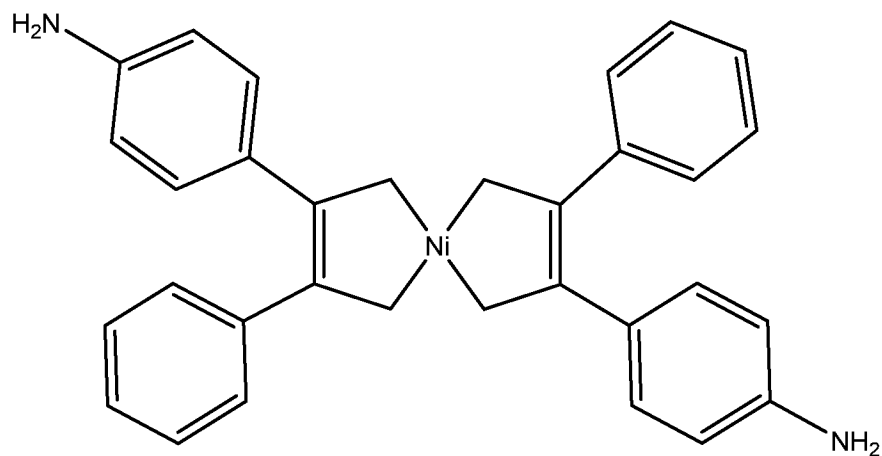
Metal dithiolene dyes/pigments
