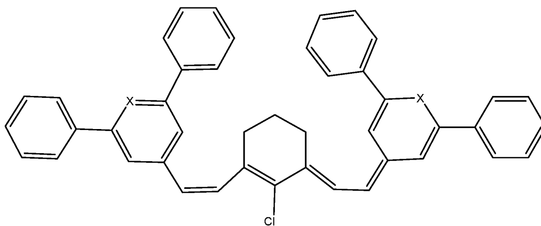
Pyrilium (X=O), thiopyrilium (X=S) dyes/pigments
