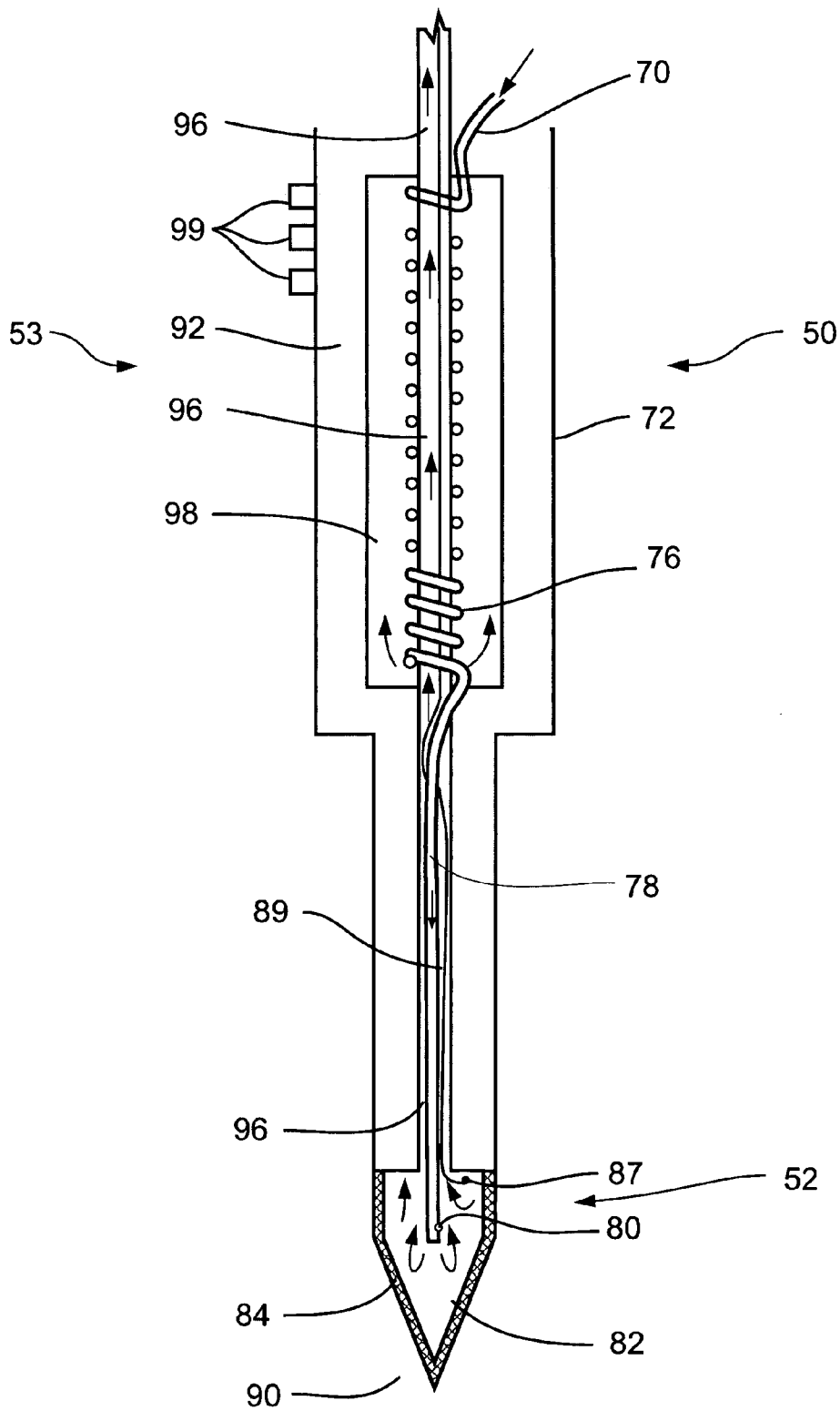
Fig. 7(Prior Art)
