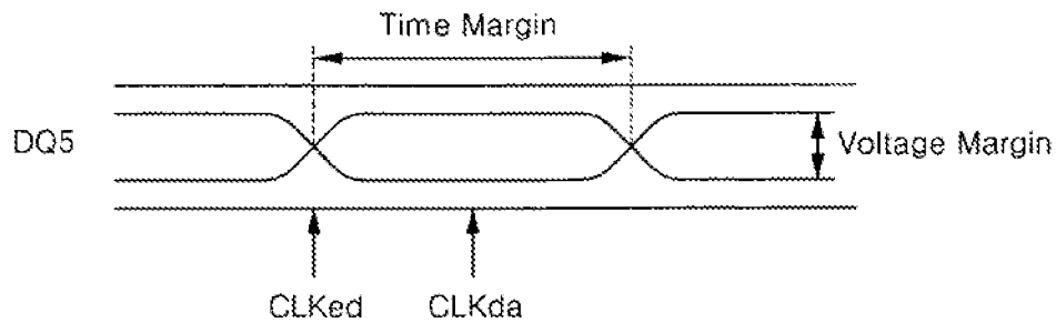
FIG. 2B (CONVENTIONAL ART)
