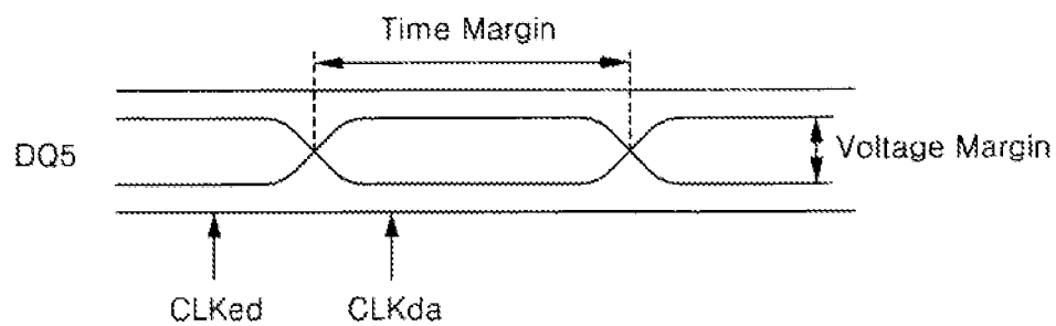
FIG. 2C (CONVENTIONAL ART)
