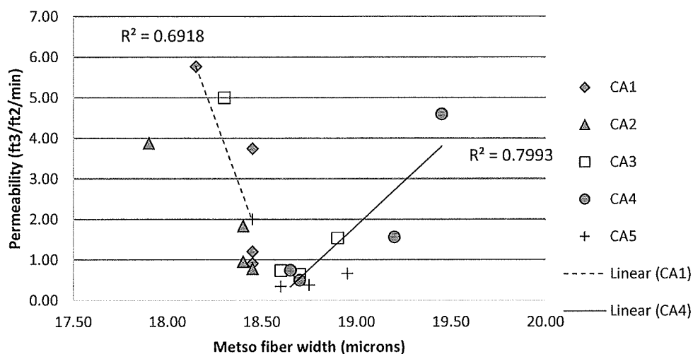
Fiber width vs Air Permeability: Method 1, Lab 1
