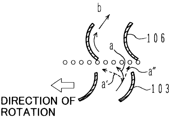
FIG.12 PRIOR ART
