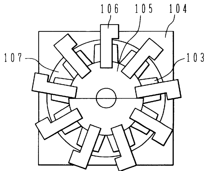
FIG.11 PRIOR ART
