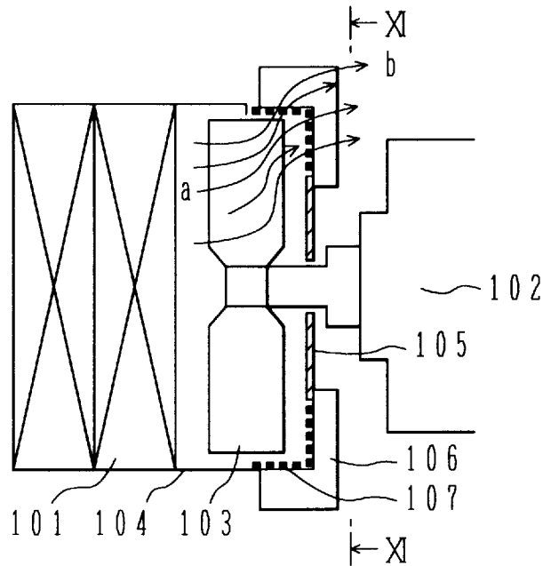
FIG.10 PRIOR ART
