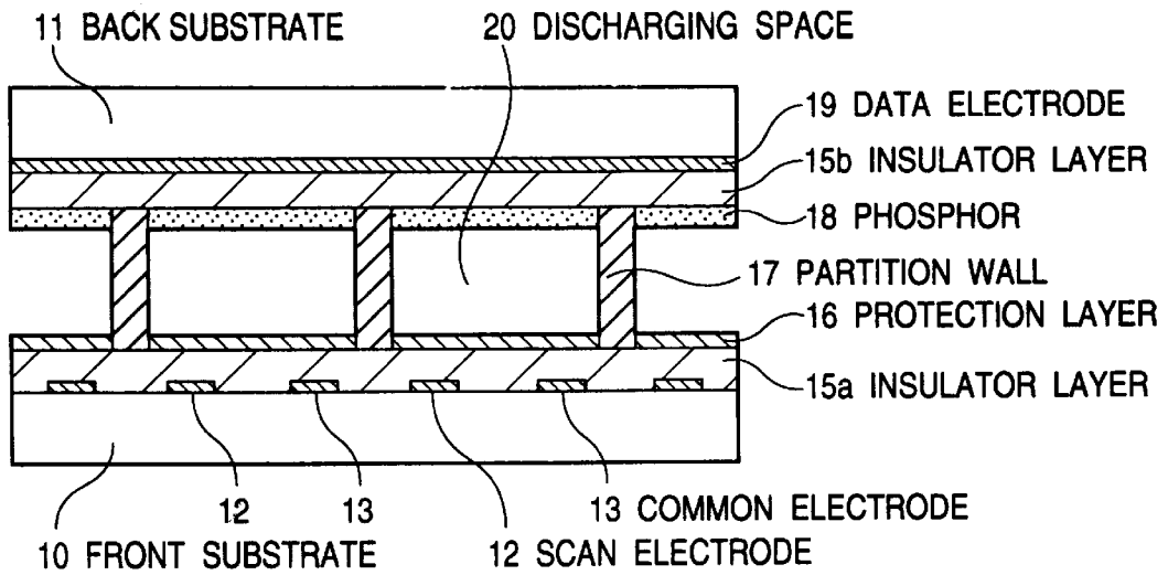
Fig. 2 PRIOR ART
