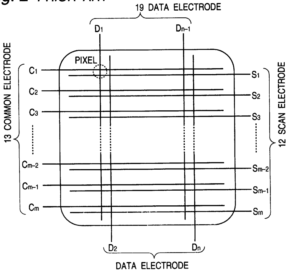
Fig. 2 PRIOR ART
