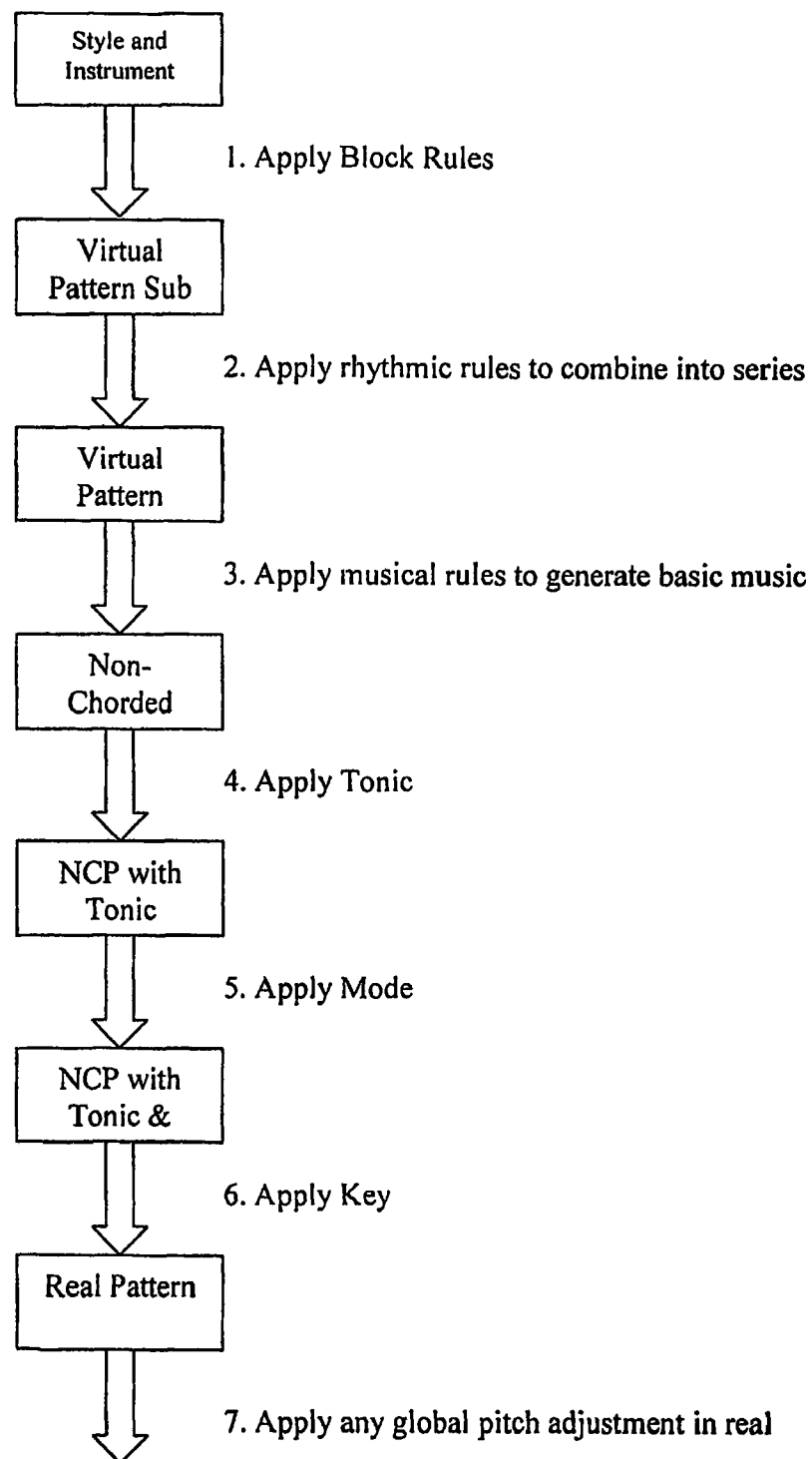
General Musical Generation Flow
