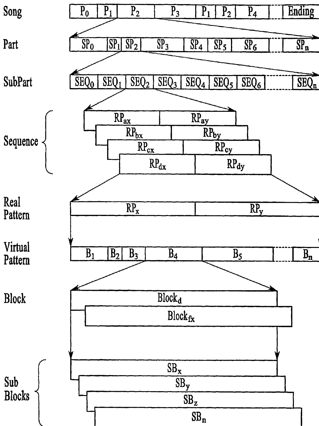
Song Structure
