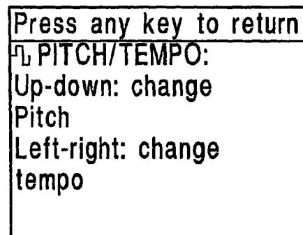
Help Screen
