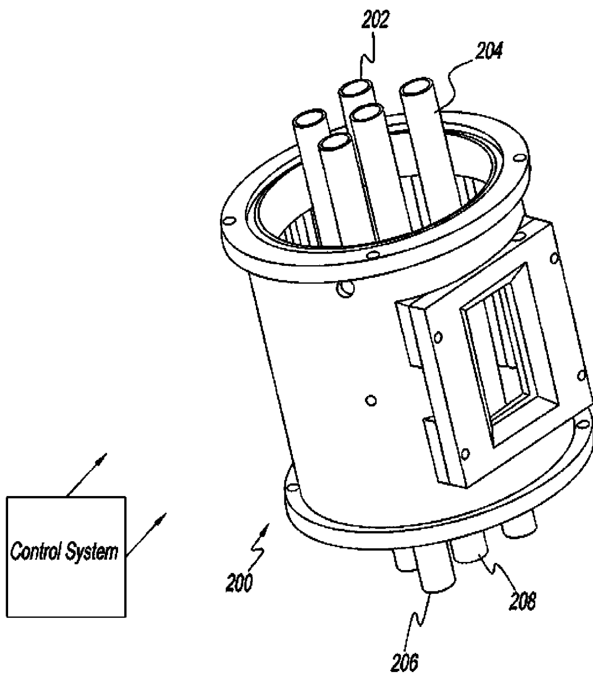
Multiple tube reactor
