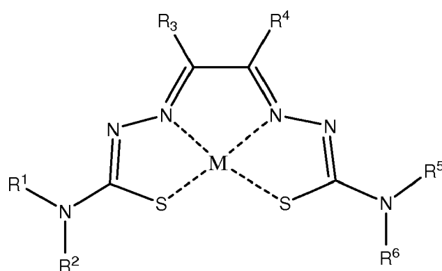
Formula (I)
