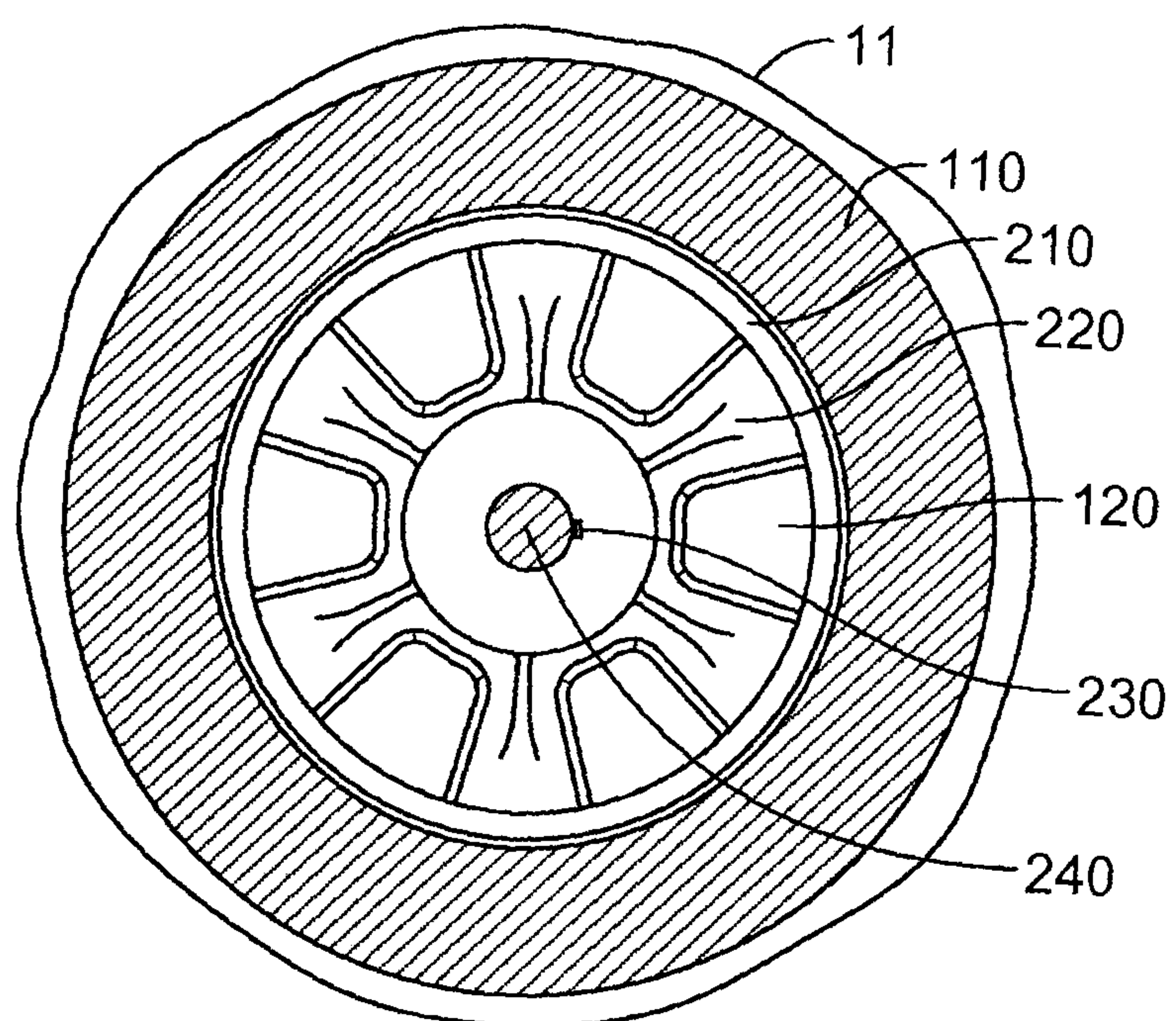
Section B-B
