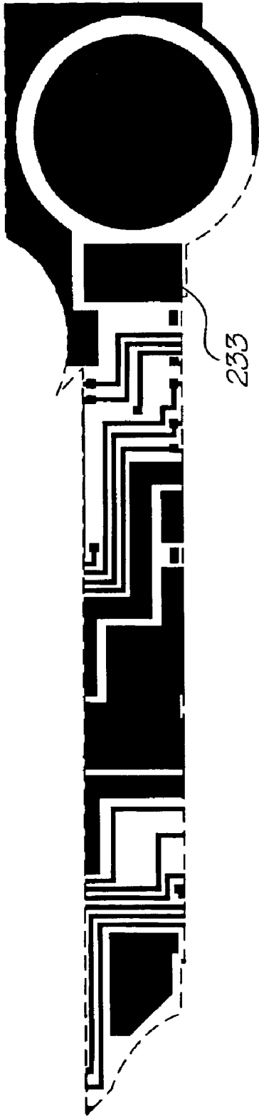
Metal 2 mask
