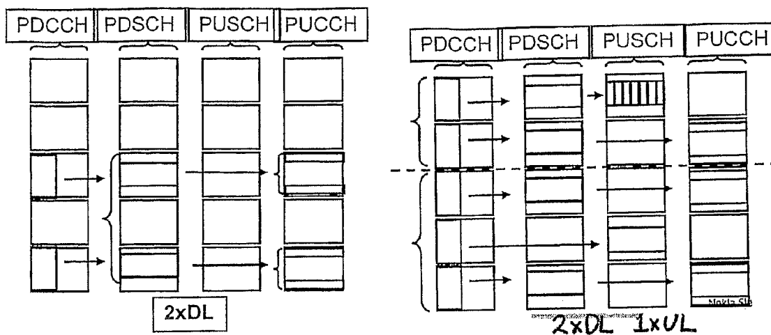
Figure 3. Different UL/DL configurations.
