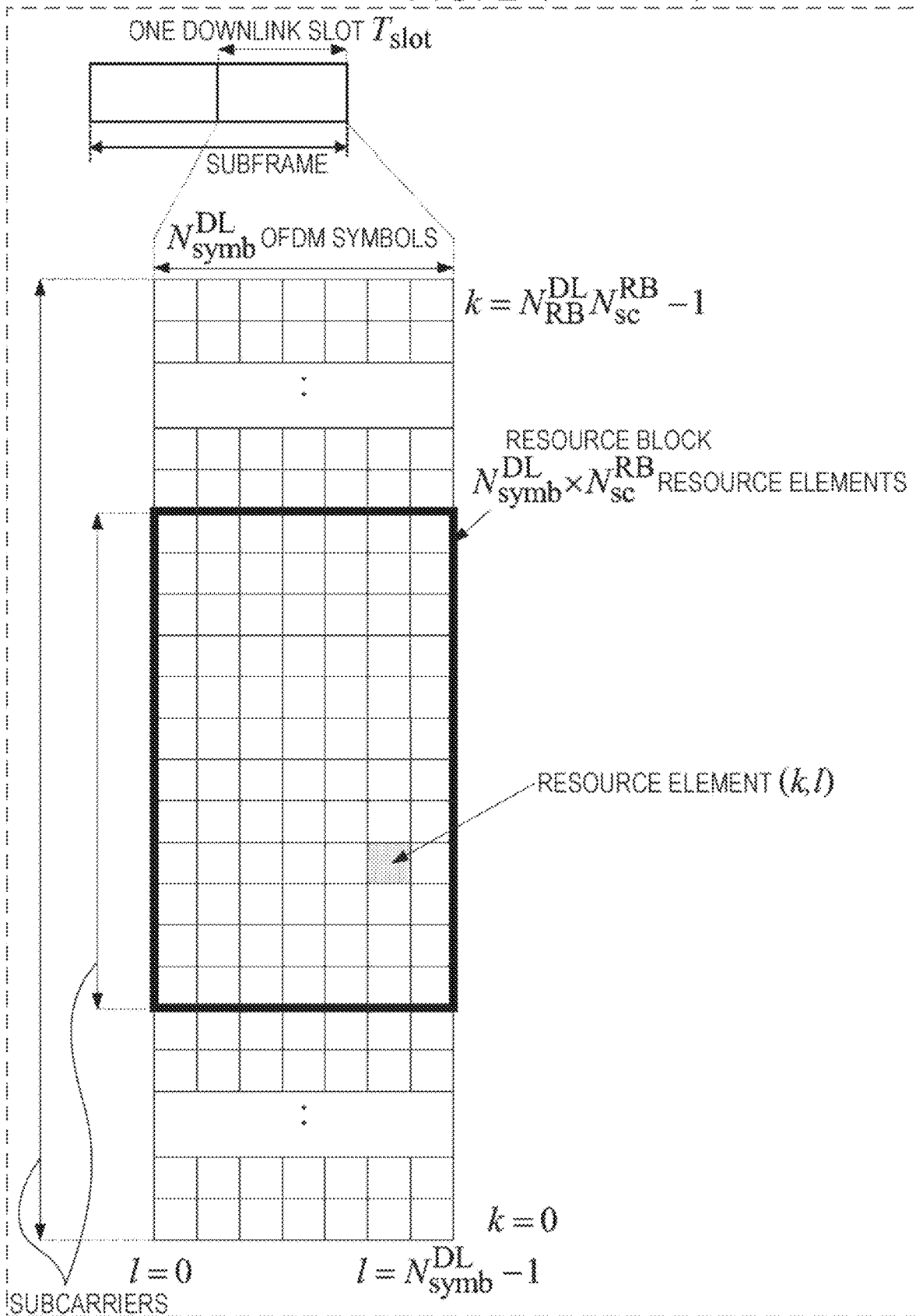
FIG. 2 (PRIOR ART)
