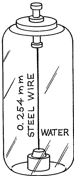
WIRE PHANTOM (SPATIAL RESOLUTION, MTF)
