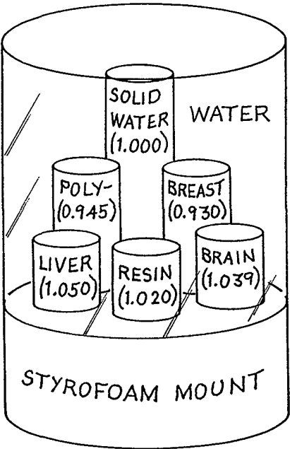
ELECTRON DENSITY PHANTOM (CONTRAST, CT LINEARITY)
