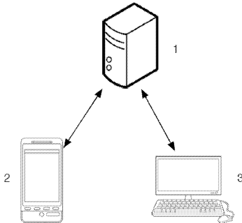
FIG. 9 One potential implementation of the secure system methodology as used in a multiple device TTS system. TTS measurements from both a mobile device and desktop computer create a security state of the two device system which is analyzed and acted upon by a enterprise wide security server.
