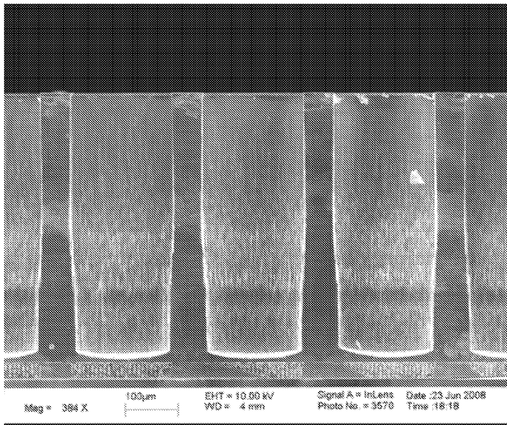
SEM image of deep etched 190umx190um openings.
