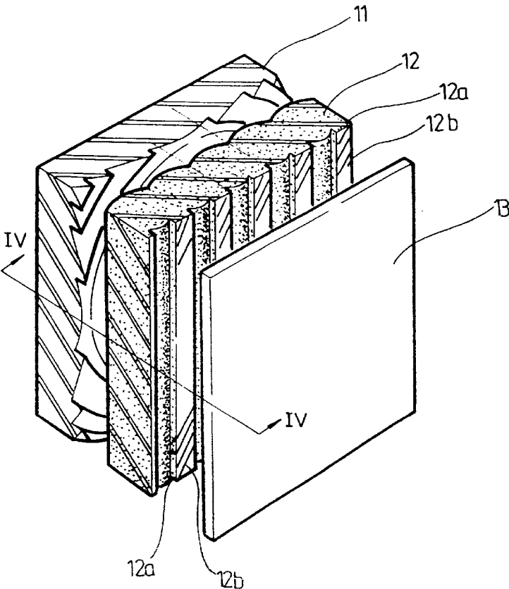
FIG. 4 (PRIOR ART)
