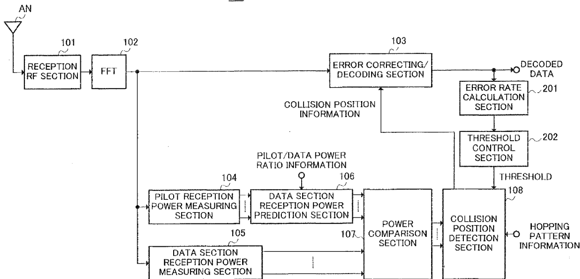
200 OFDM RECEPTION APPARATUS
