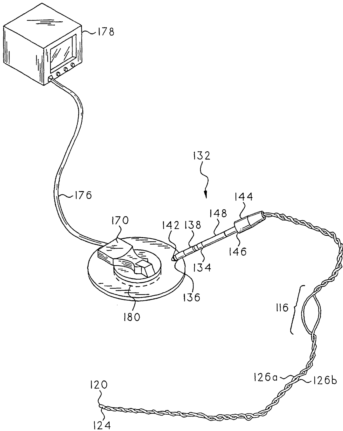
FIG. 7 (Prior Art)
