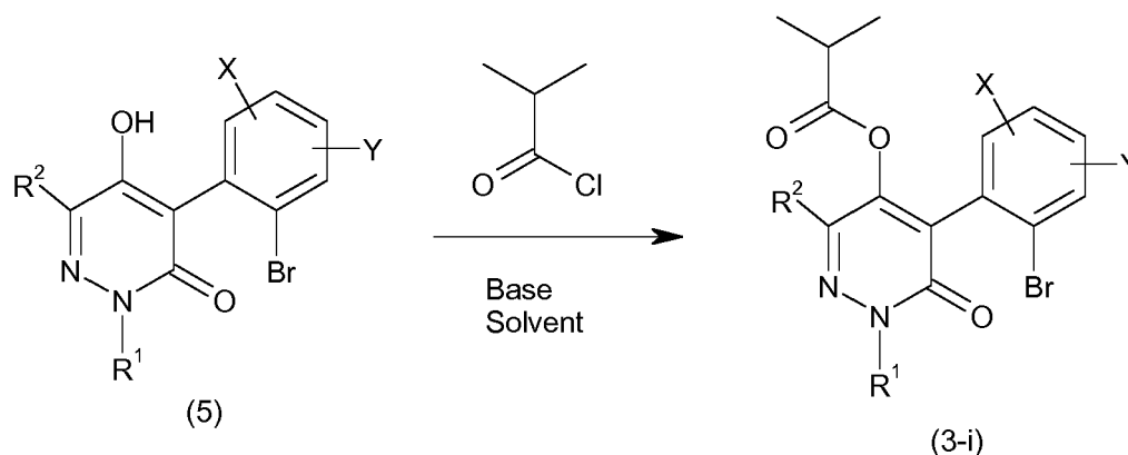
Reaction scheme 3
