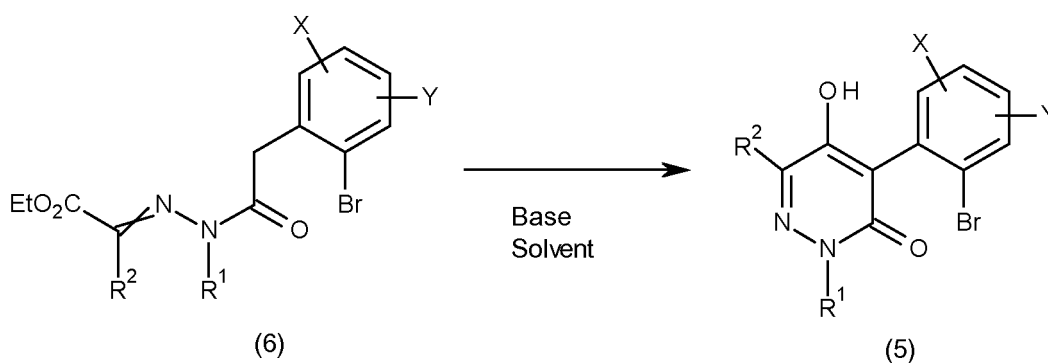
Reaction scheme 4
