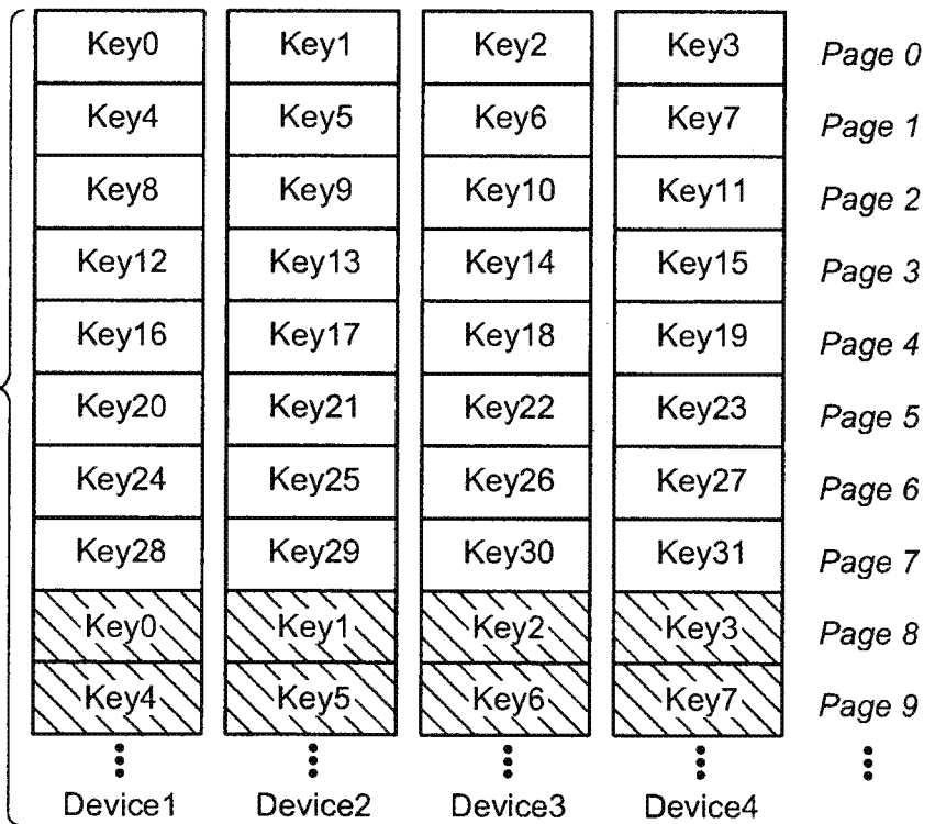
32 Keys Applied to 8 Pages in Each Device
