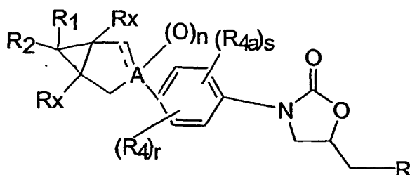
Formula II
