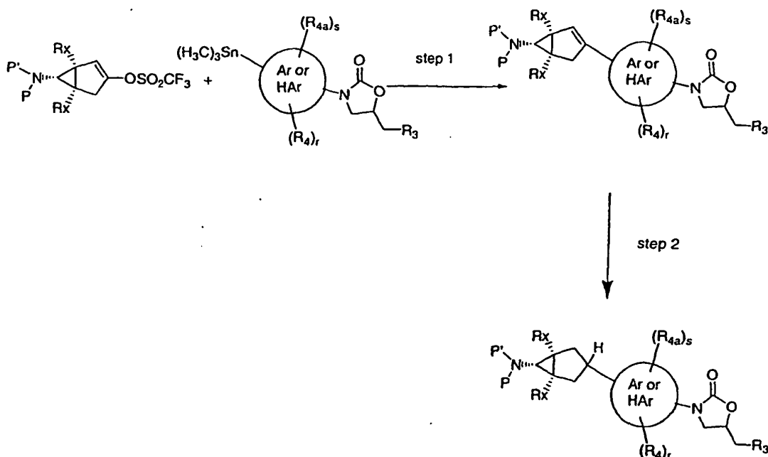
Scheme V
