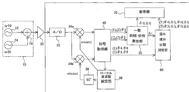
70 DISPLAY UNIT 40 PHASE ACQUISITION UNIT 50 MATCH TIME/PHASE MEASUREMENT UNIT 60 DISTORTION COMPONENT PHASE MEASUREMENT UNIT 36 LOCAL FREQUENCY SETTING UNIT
