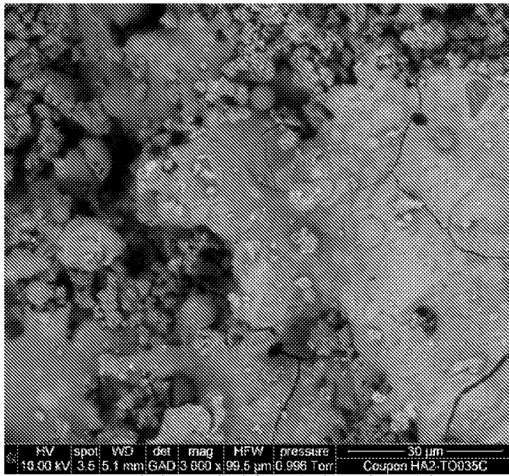
Figure 7: HA2-TO035C backscatter, detail of silver distribution showing "light grey" patchy areas, composed of nano-scale silver-rich features
