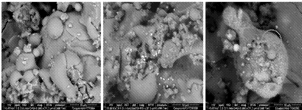
Figure 4a: HA Control - TQ035A backscatter
