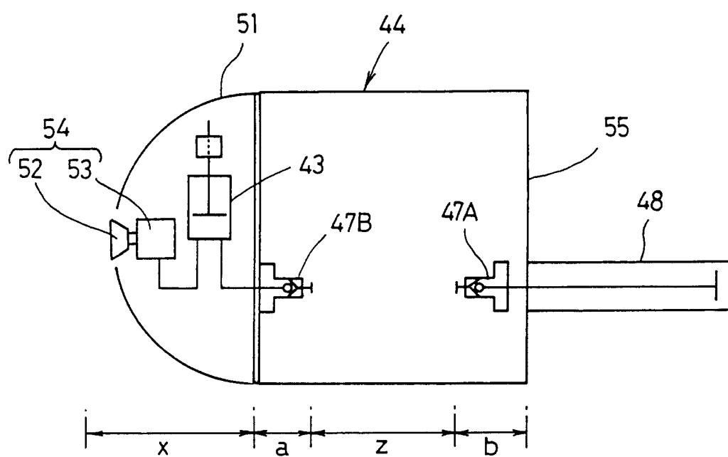
FIG. 5 (PRIOR ART)
