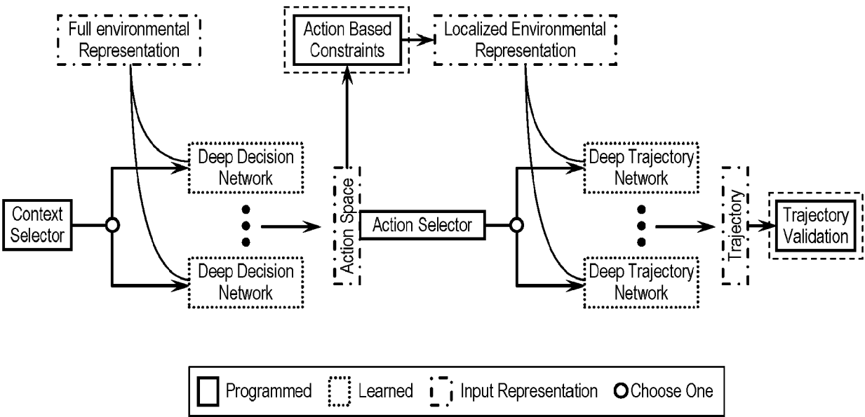
Architecture of Safety confined Hybrid Trajectory Generator
