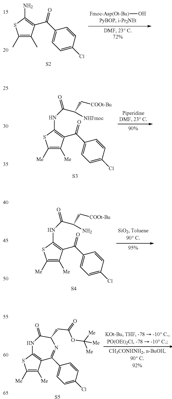
Scheme S2. Synthesis of enantiomerically enriched (+)-JQ1.
