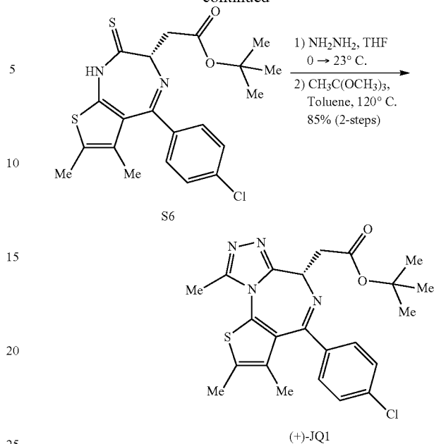
Scheme S1. Synthesis of the racemic bromodomain inhibitor ( \pm )-JQ1.
