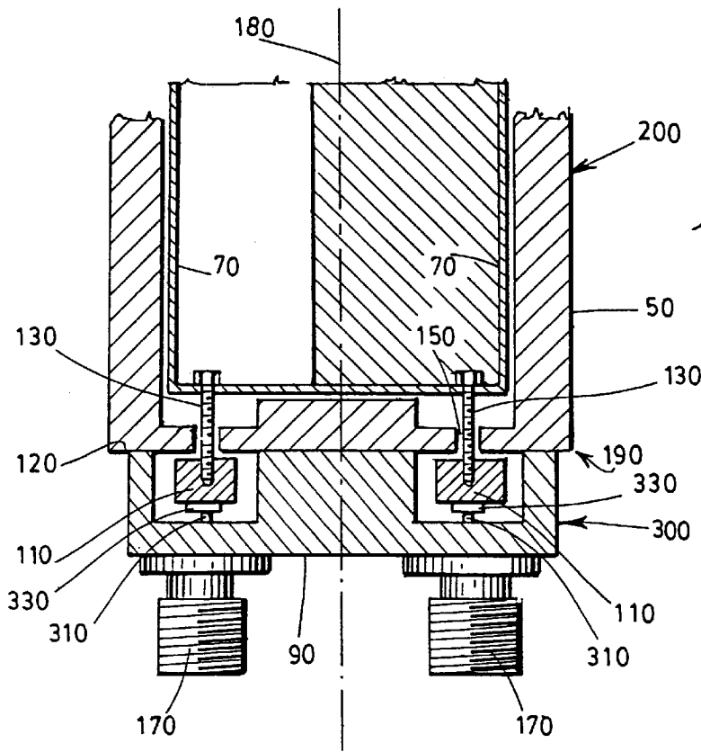
FIG. 1 (PRIOR ART)
