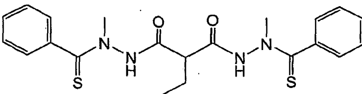
Compound (5)
