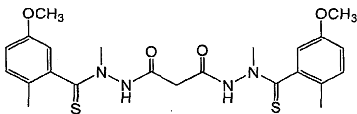
Compound (13)
