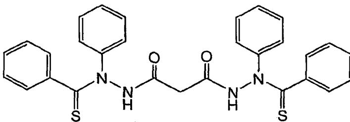
Compound (3)
