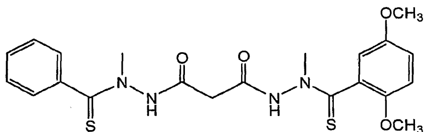
Compound (15)
