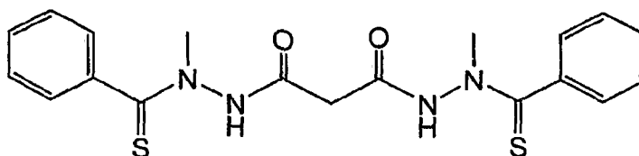
Compound (1)
