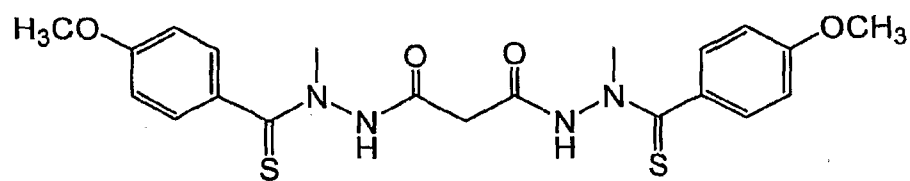
Compound (6)
