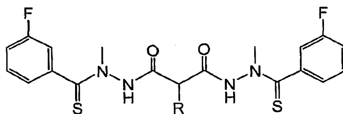
Compound (10)
