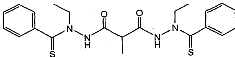
Compound (16)
