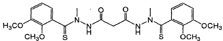
Compound (11)
