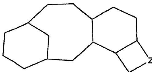
(IX)
