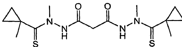
Compound (17)
