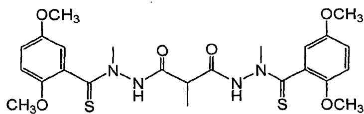
Compound (9)
