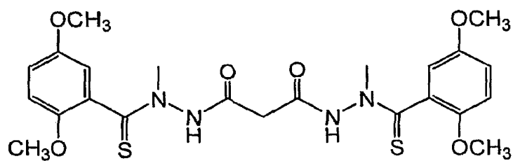
Compound (8)
